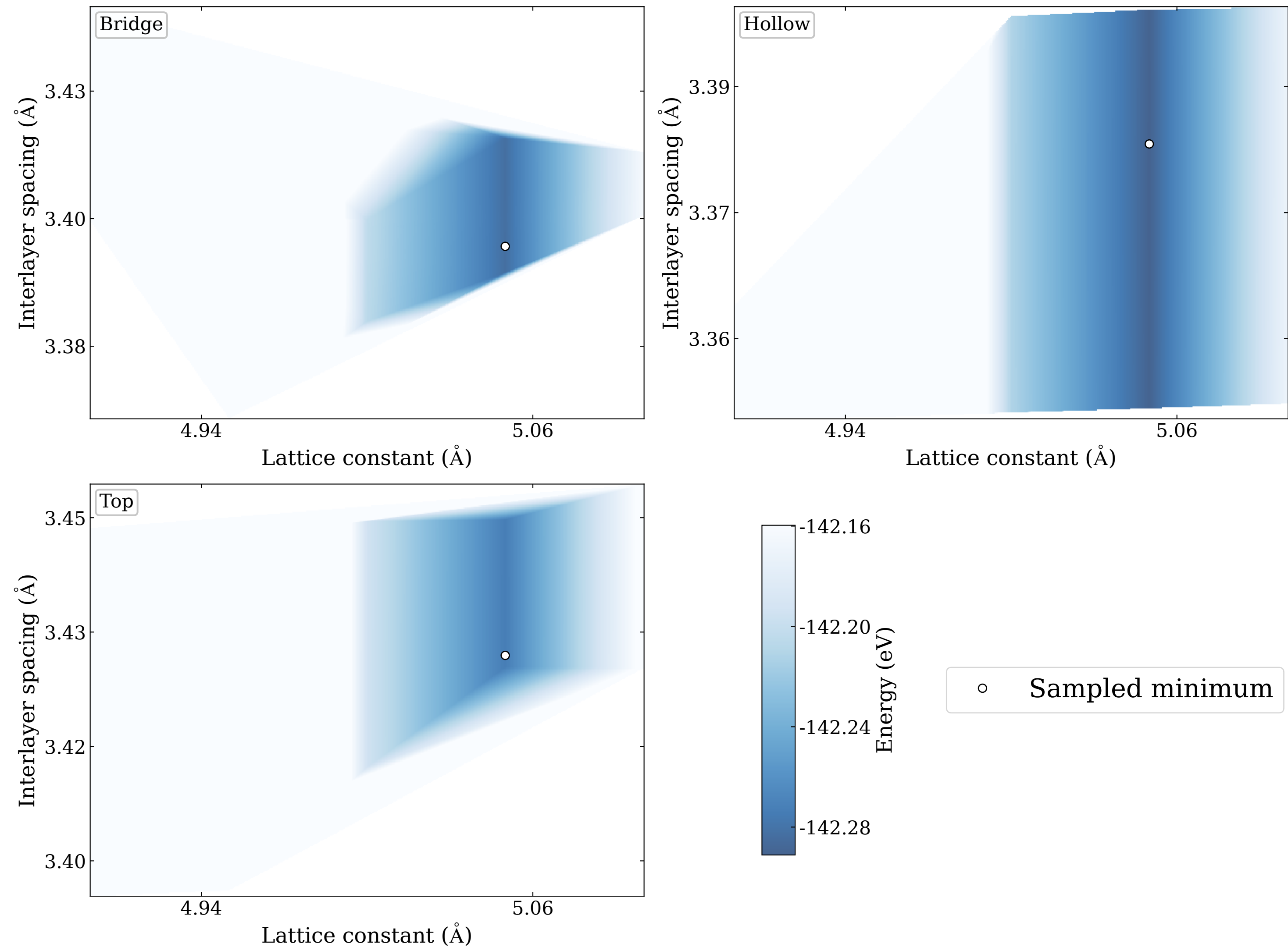
Total energy versus lattice and interlayer spacing for Graphene-BC 3
