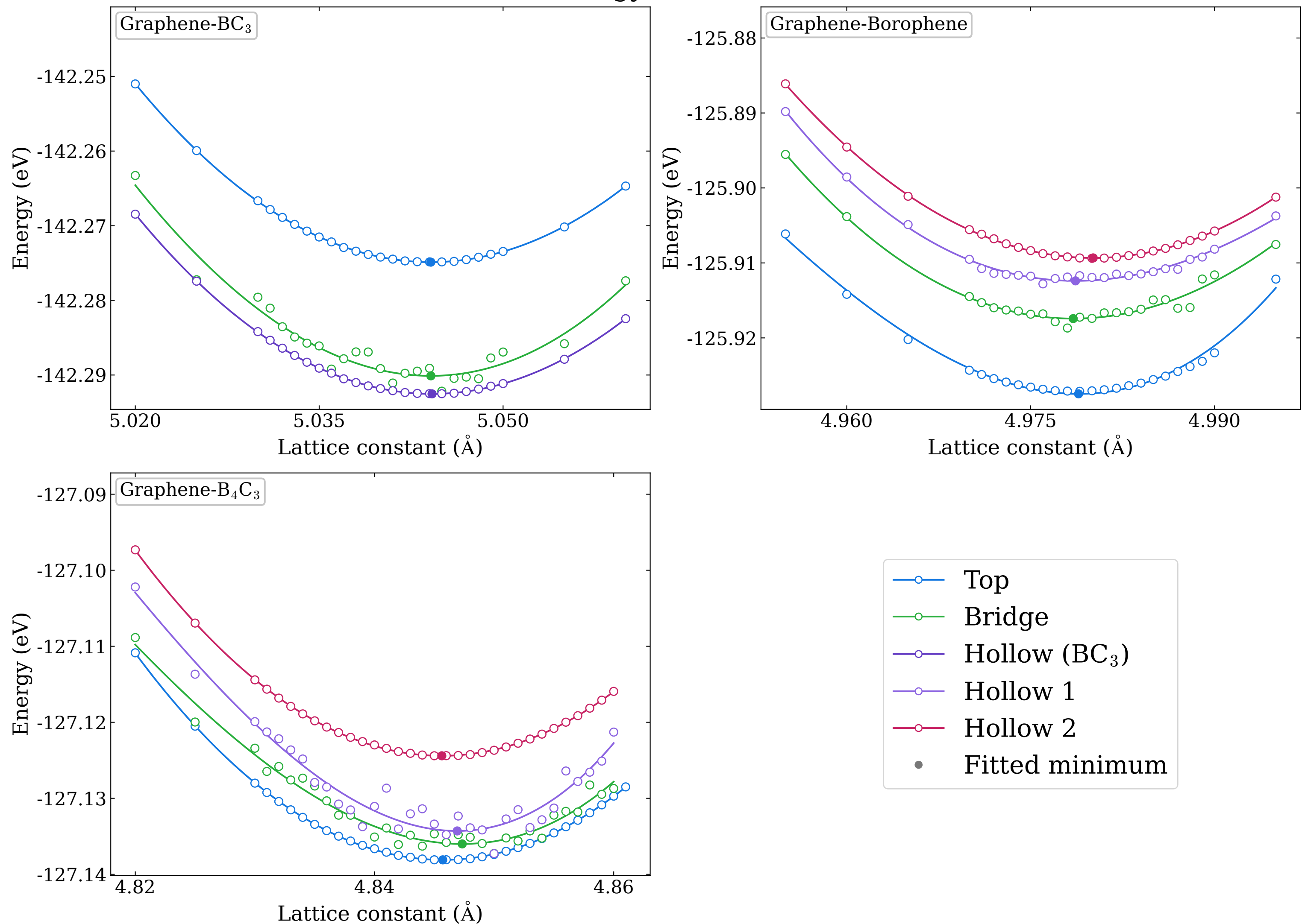
Total energy versus lattice
