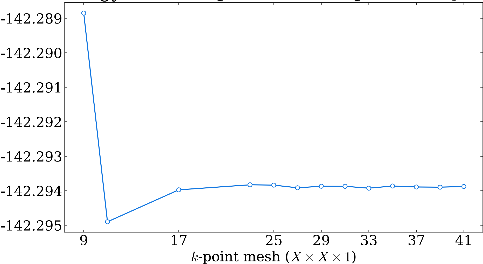
Total energy versus k-points for Graphene-BC 3 (H)
