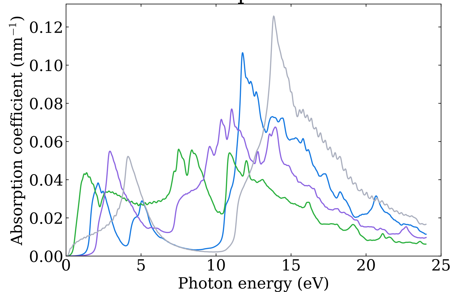
Absorption coefficient for monolayers by PBE
