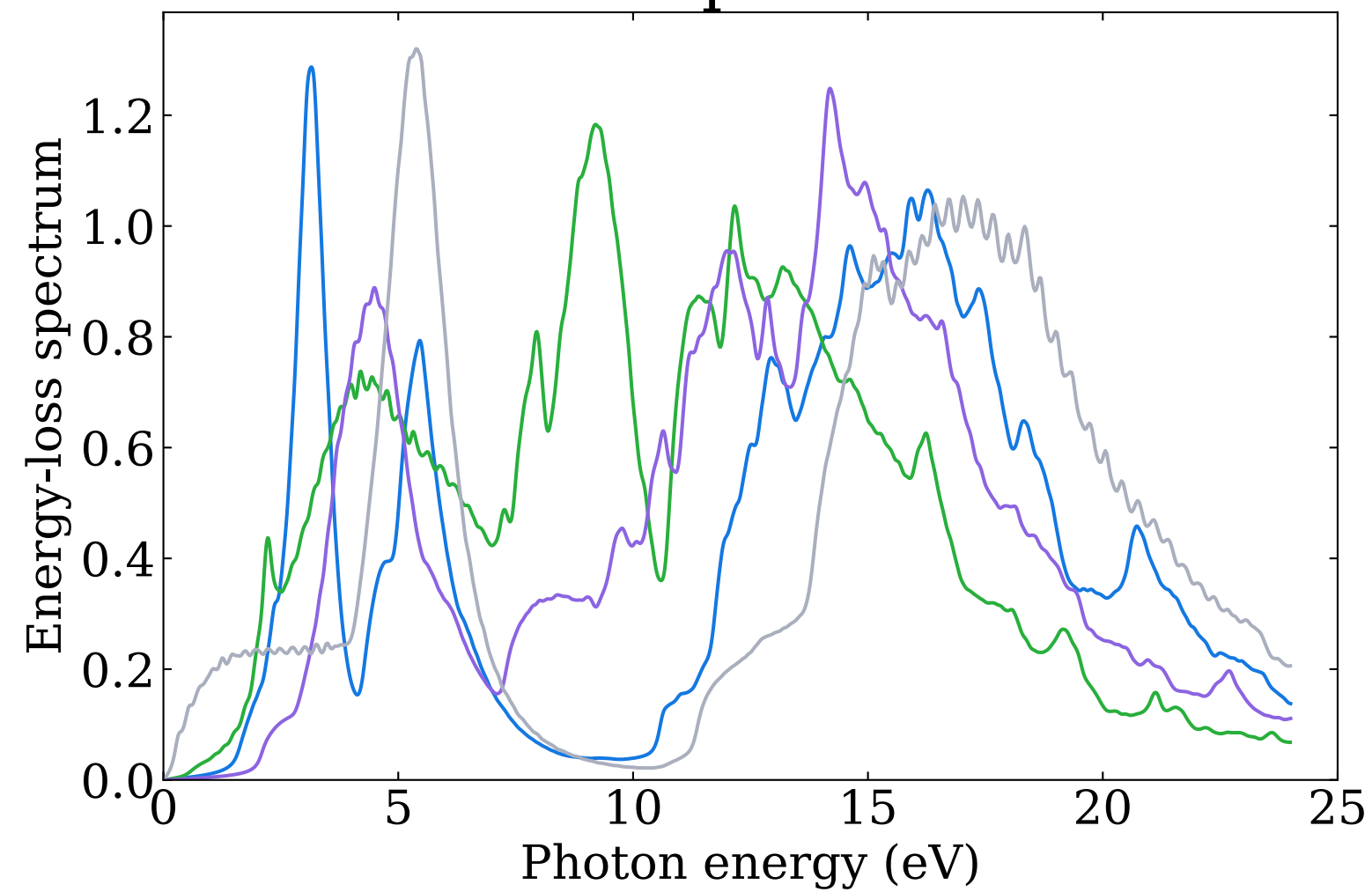
Energy-loss spectrum for monolayers by PBE
