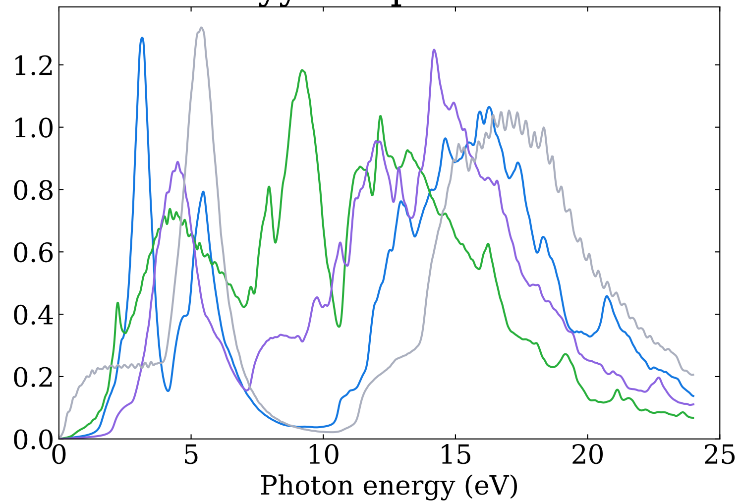
Energy-loss spectrum for monolayers by PBE
