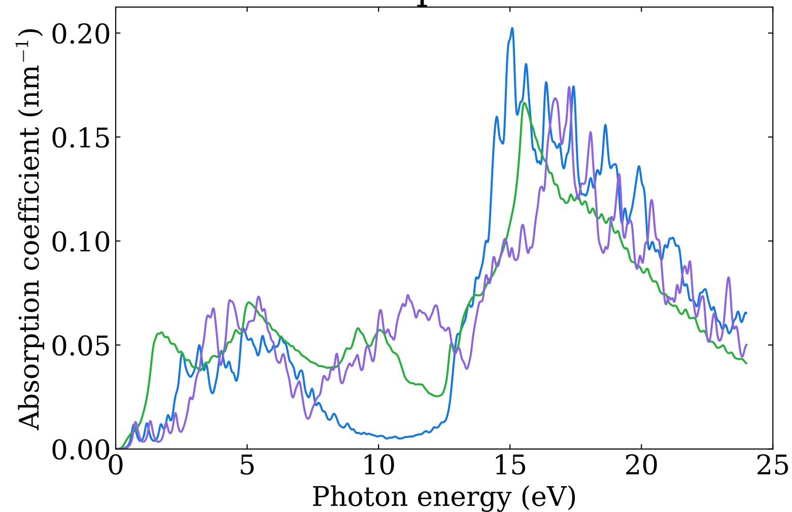
Absorption coefficient for bilayers by HSE06
