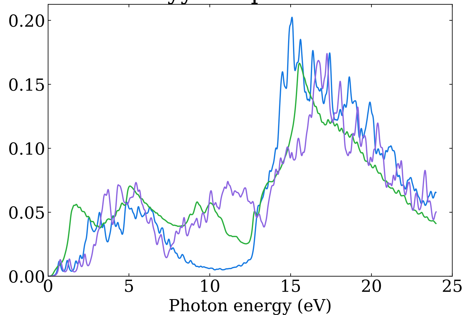
Absorption coefficient for bilayers by HSE06
