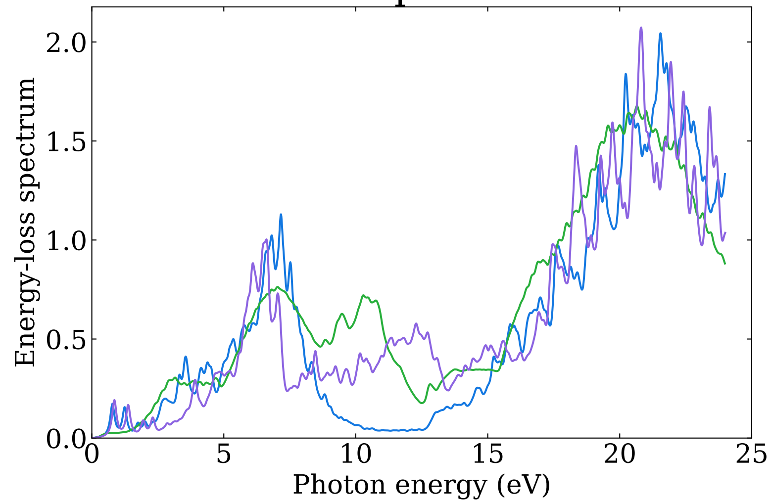
Energy-loss spectrum for bilayers by HSE06
