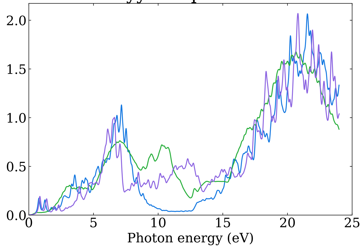
Energy-loss spectrum for bilayers by HSE06
