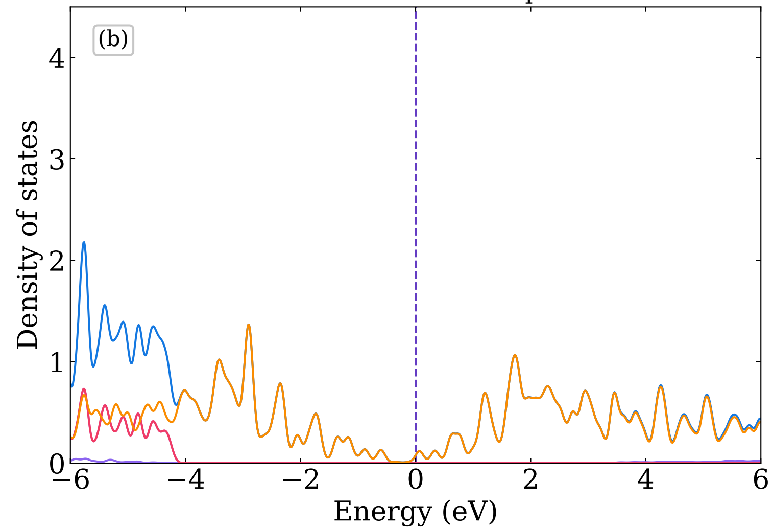
PDoS for Carbon in Graphene
