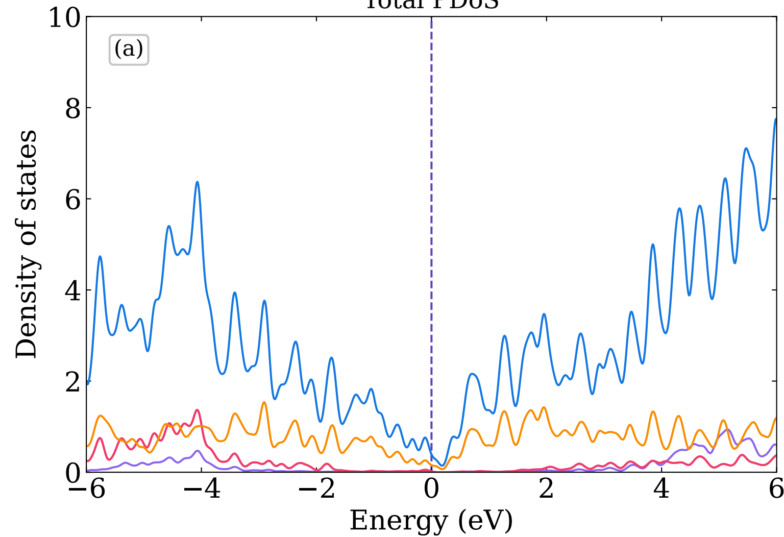
PDoS for Boron in Borophene
