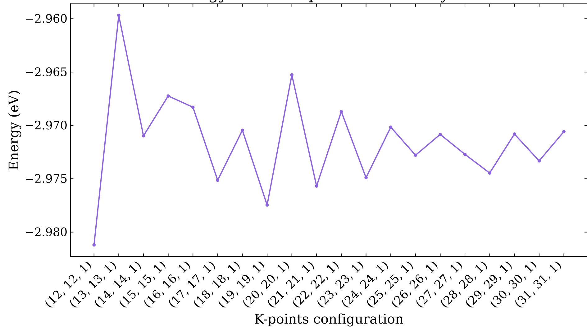
Energy versus k-points for a-Beryllene
