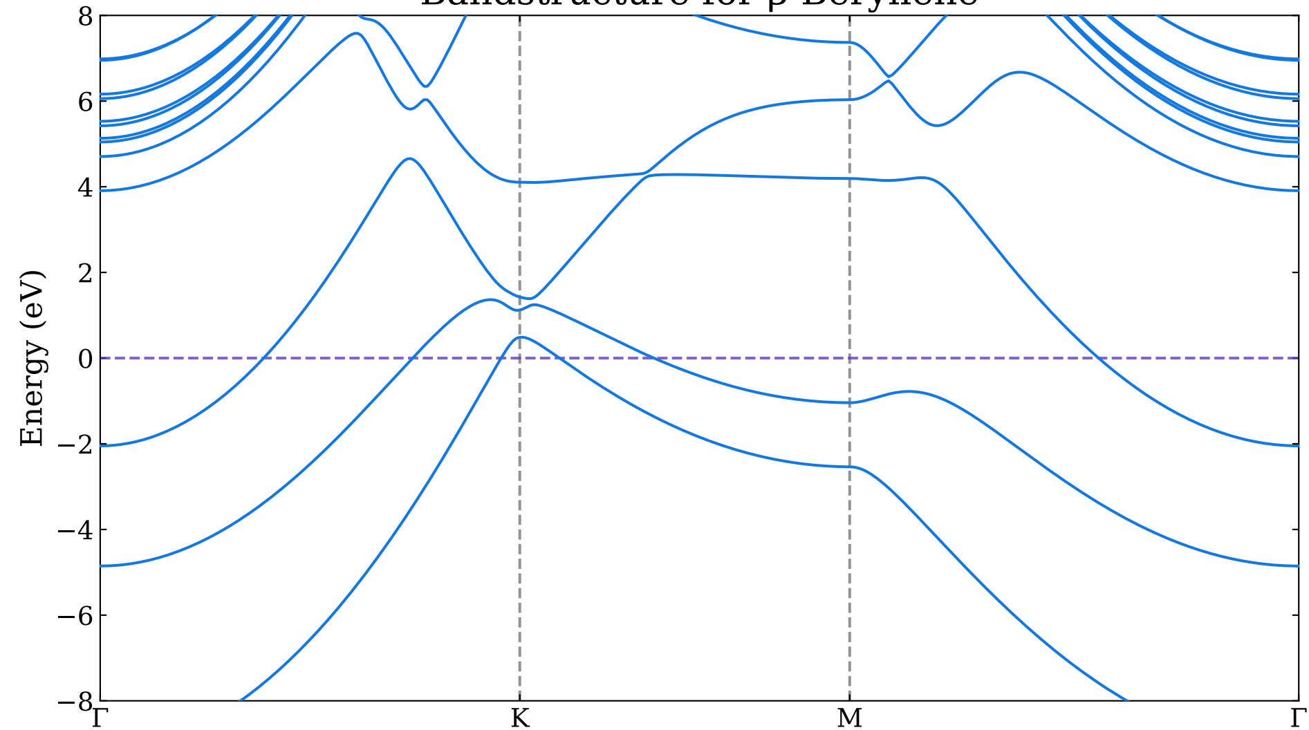
Bandstructure for \beta -Beryllene
