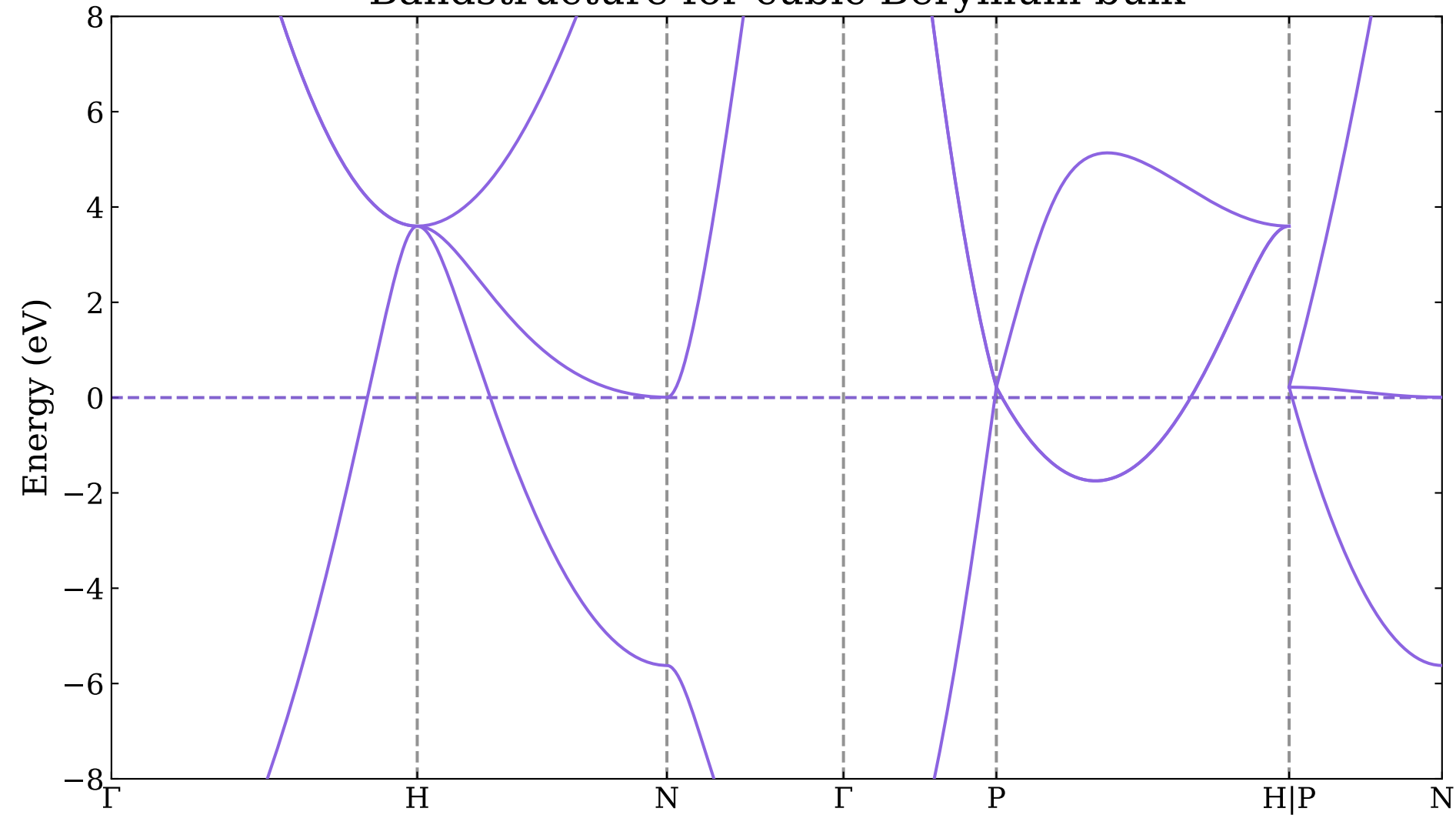
Bandstructure for cubic Beryllium bulk
