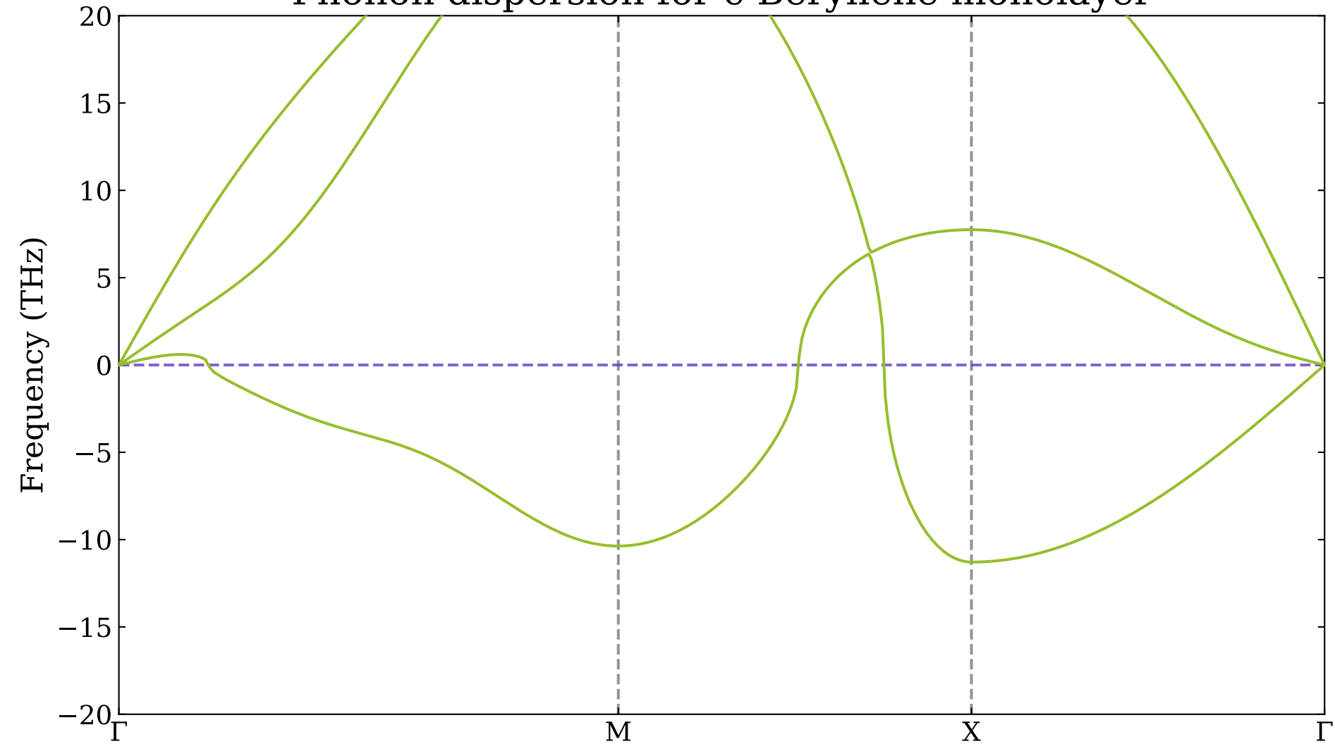
Phonon dispersion for c-Beryllene monolayer
