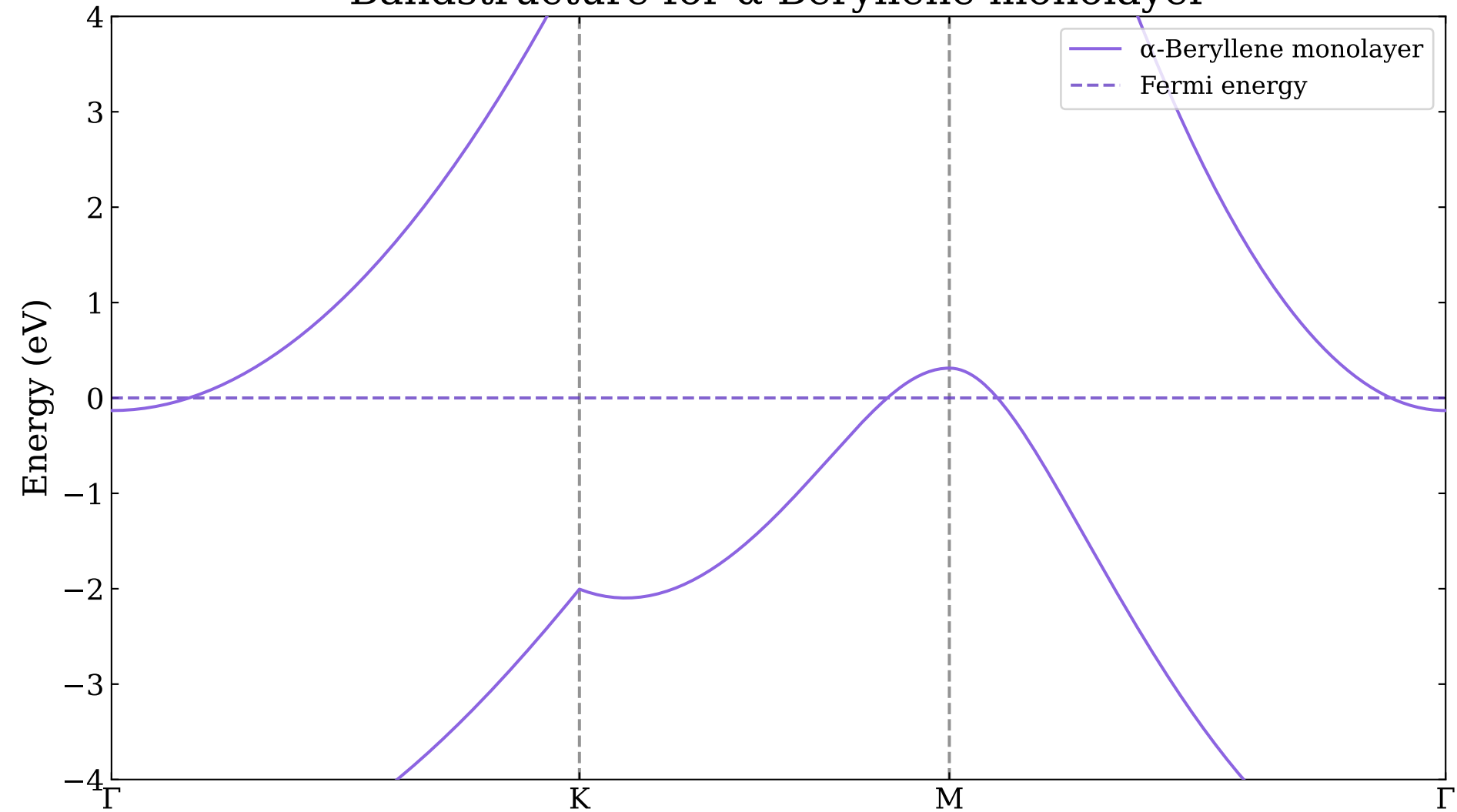
Bandstructure for \alpha -Beryllene monolayer
