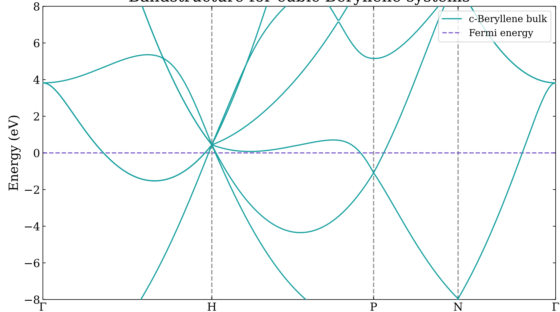
Bandstructure for cubic Beryllene systems
