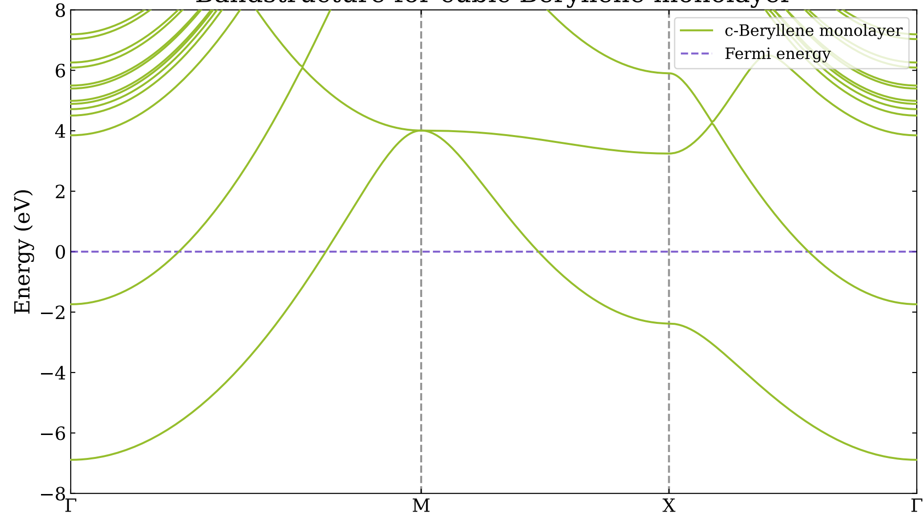
Bandstructure for cubic Beryllene monolayer
