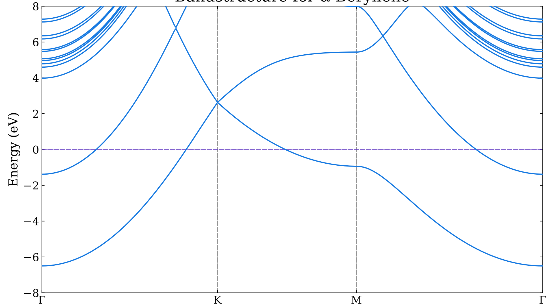
Bandstructure for \alpha -Beryllene
