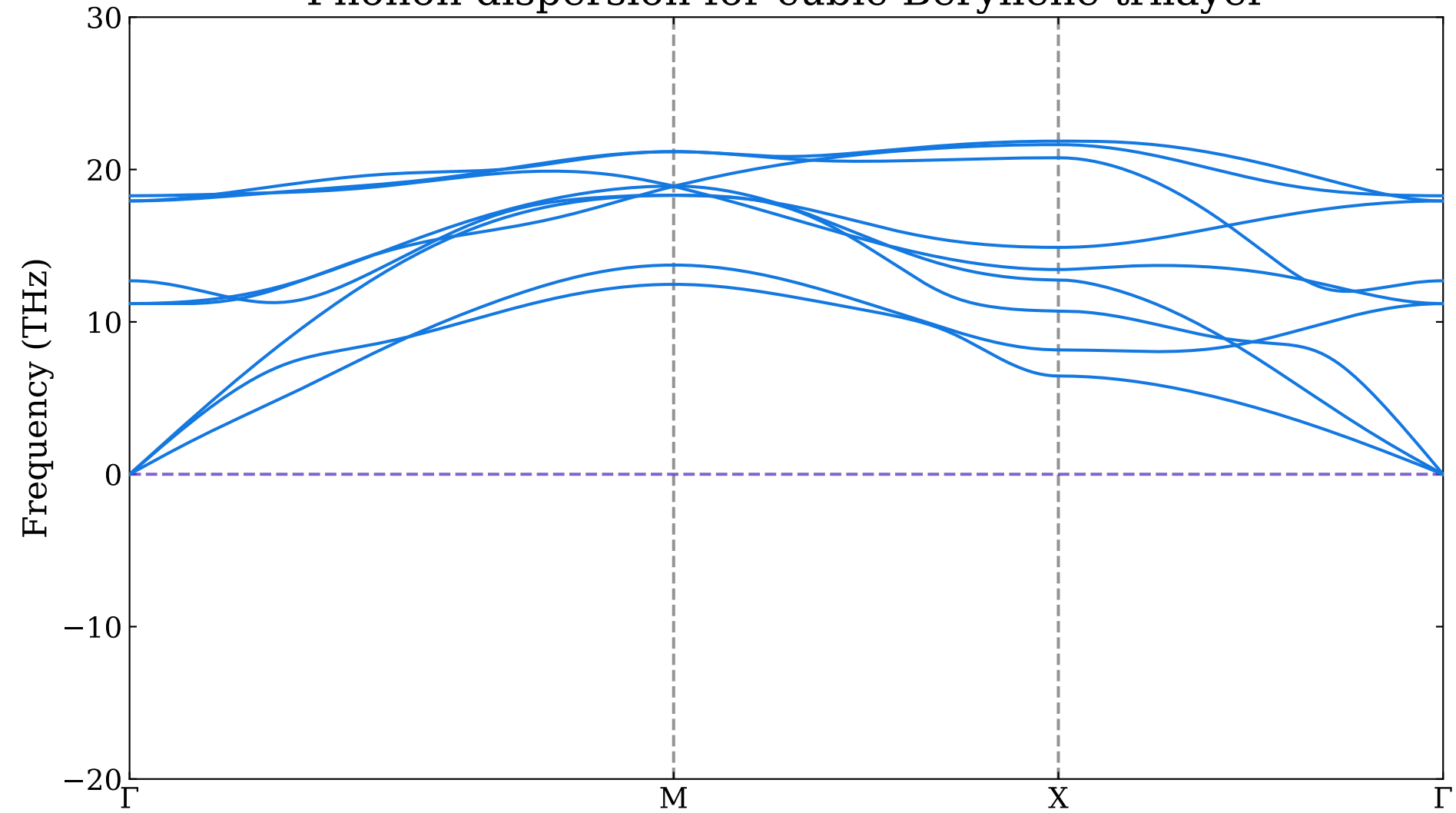
Phonon dispersion for cubic-Beryllene trilayer
