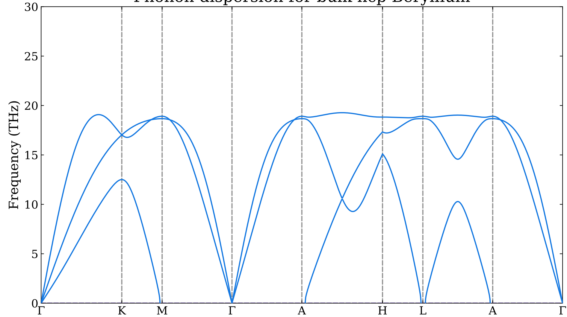
Phonon dispersion for bulk hcp Beryllium
