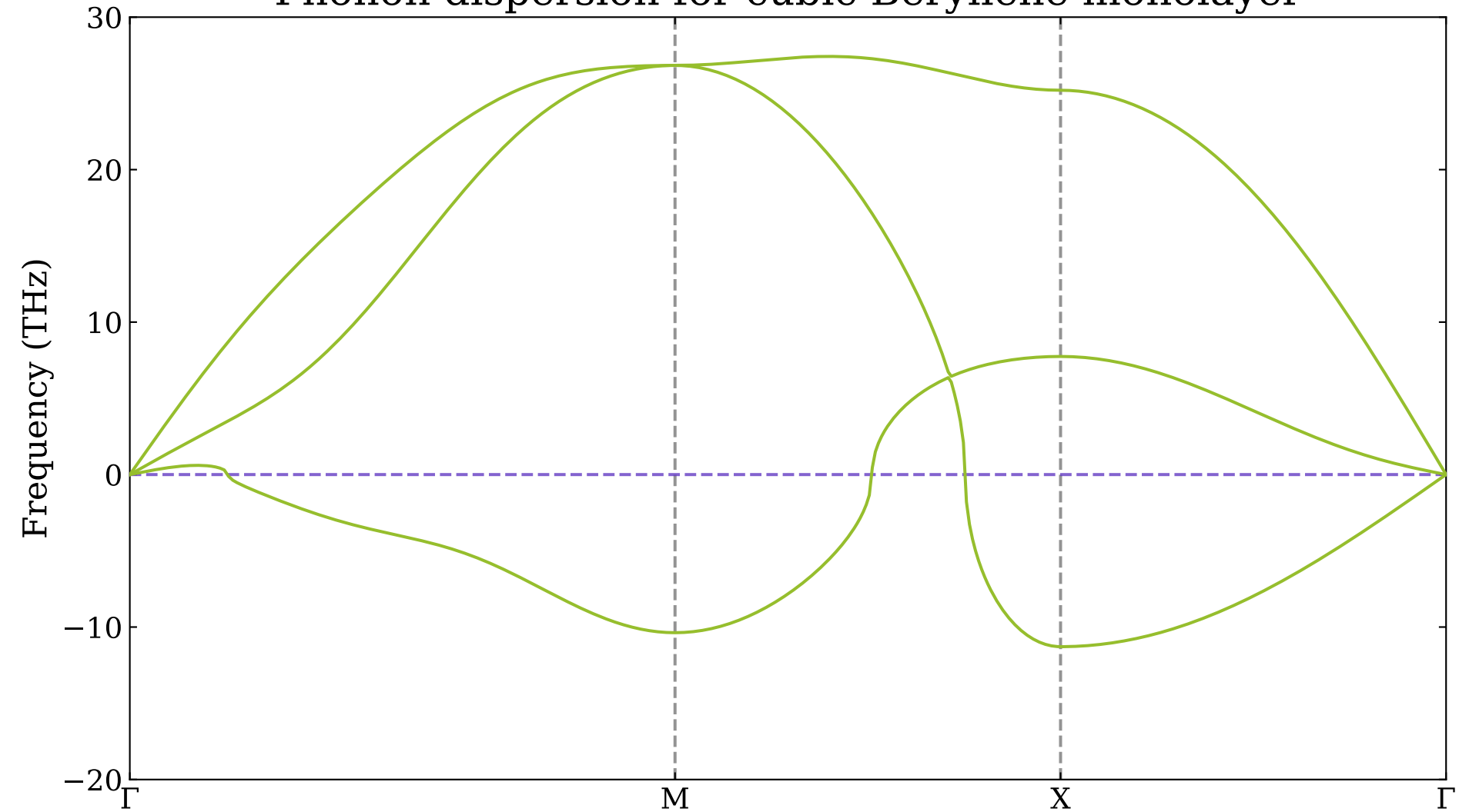
Phonon dispersion for cubic Beryllene monolayer
