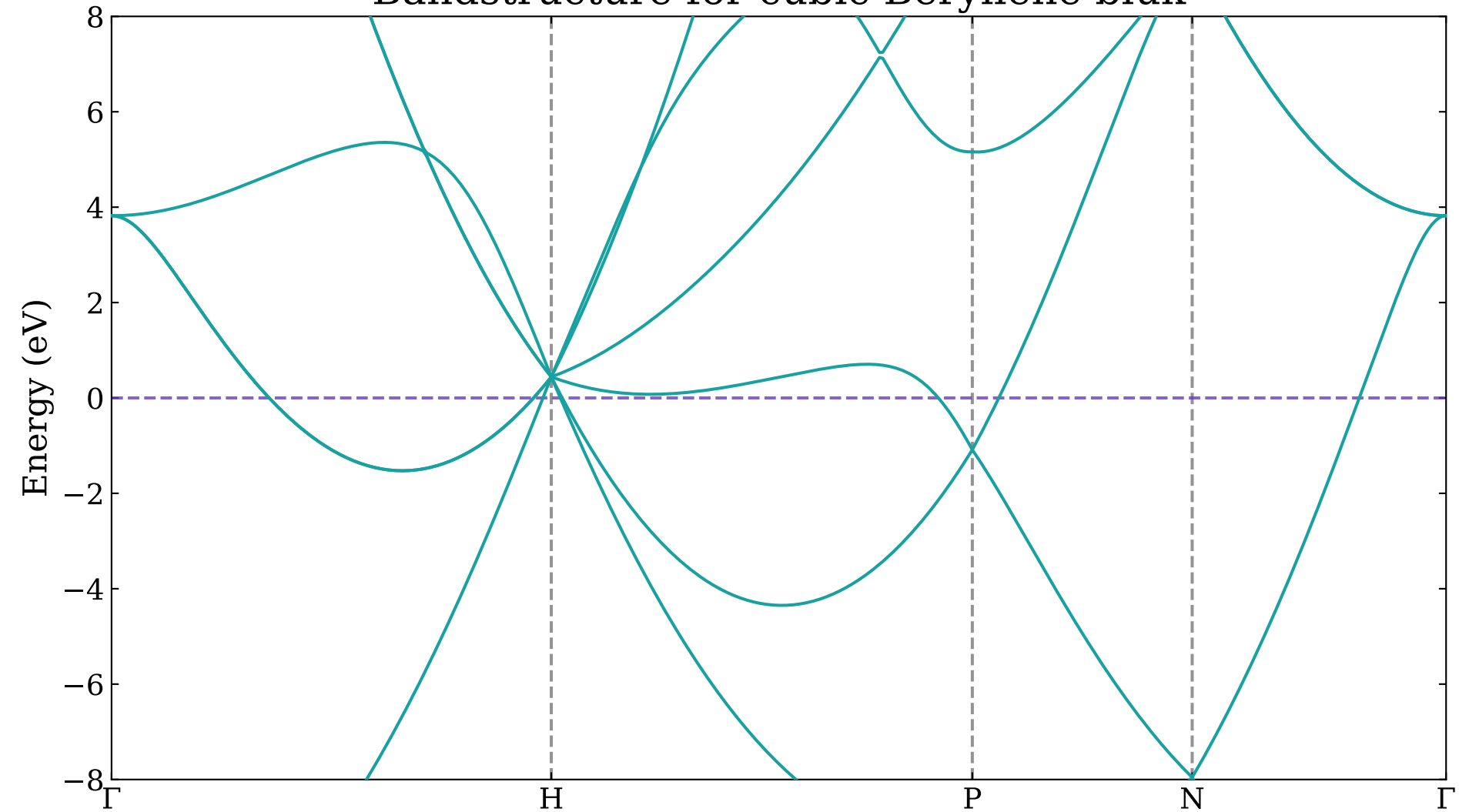
Bandstructure for cubic Beryllene bluk
