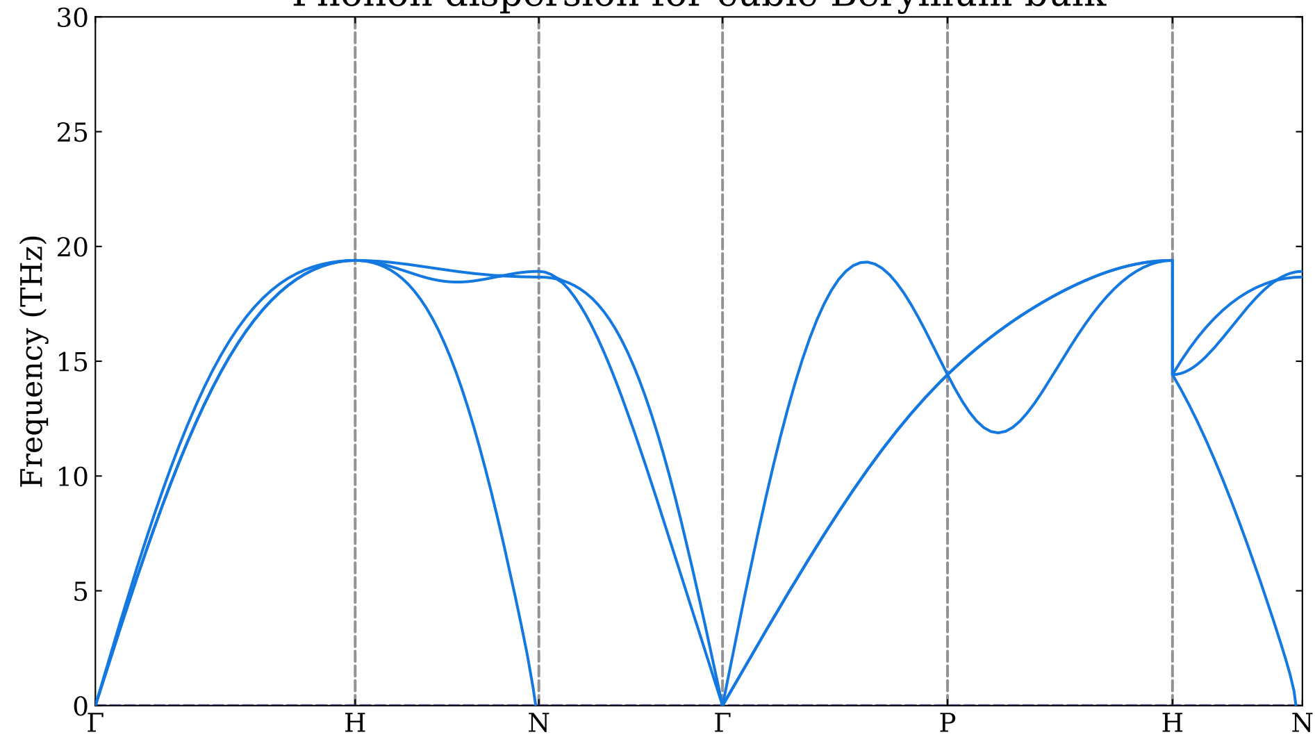
Phonon dispersion for cubic-Beryllium bulk
