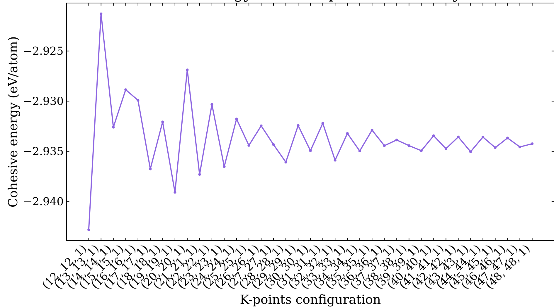
Cohesive energy versus k-points for a-Beryllene
