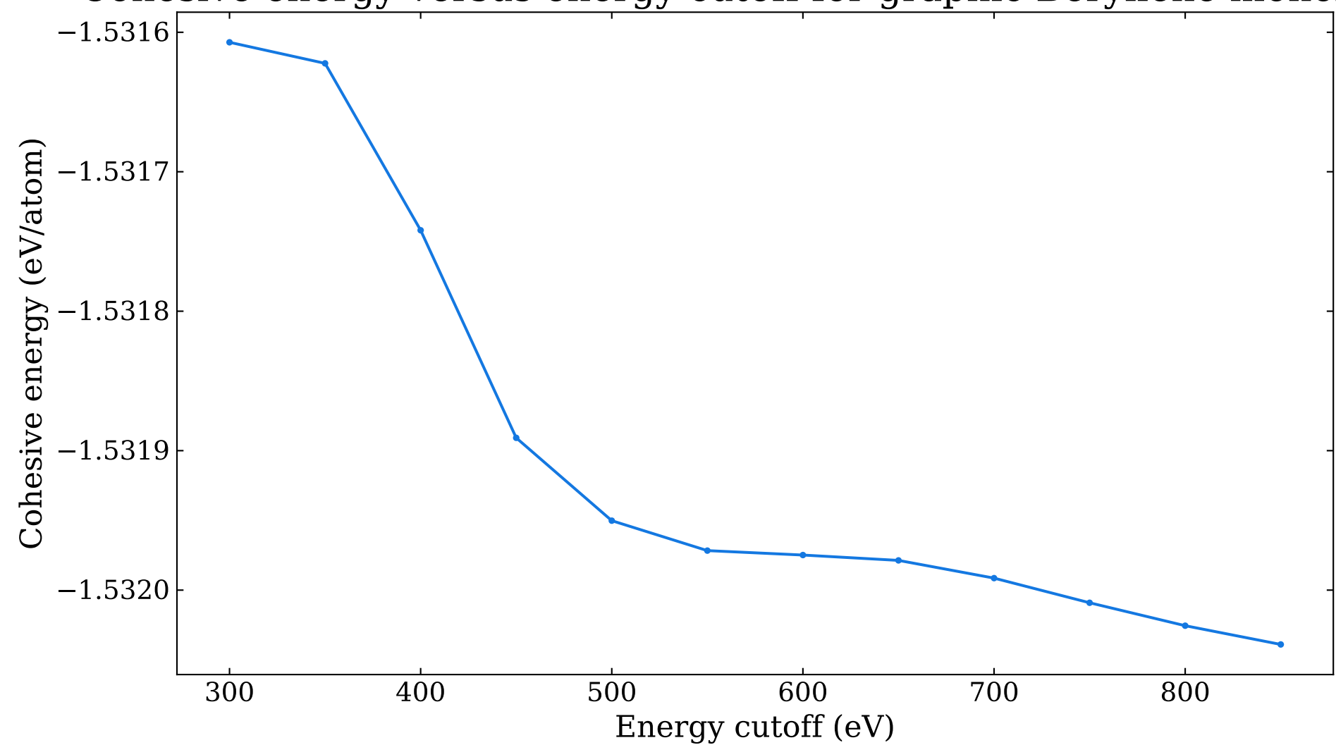
Cohesive energy versus energy cutoff for graphic Beryllene monola
