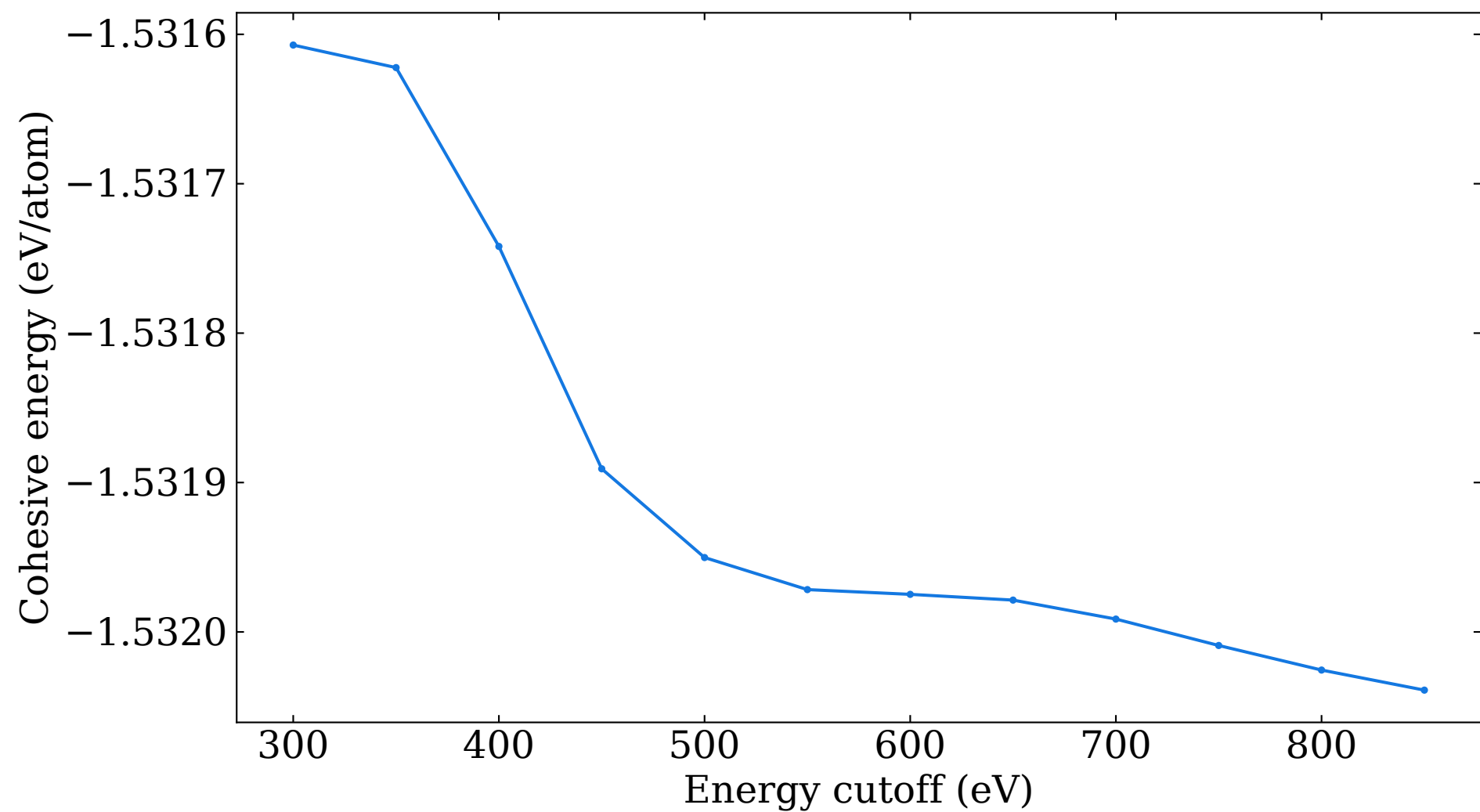
Cohesive energy versus energy cutoff for graphic Beryllene monolayer
