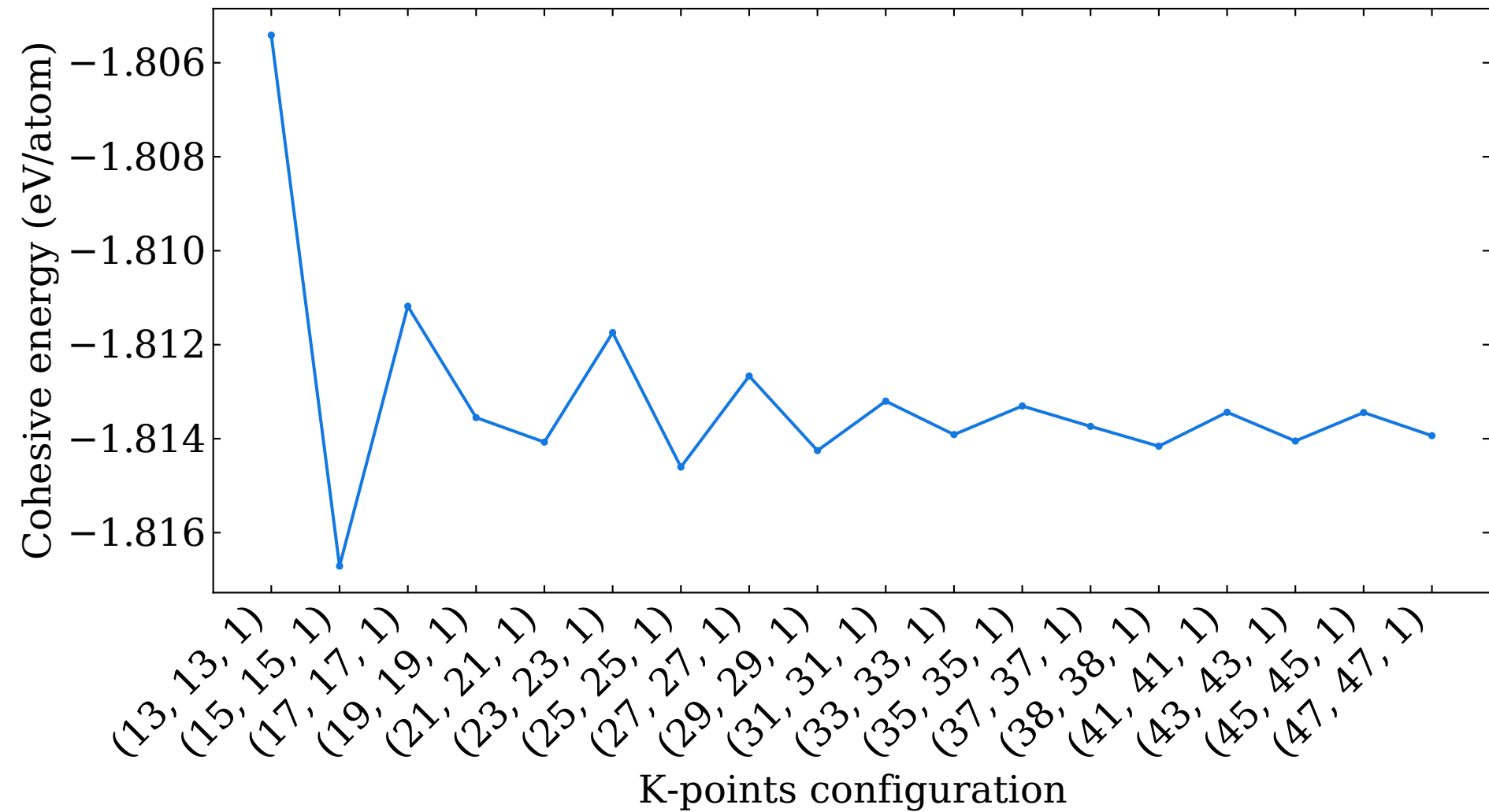
Cohesive energy versus k-points for c-beryllene monolayer
