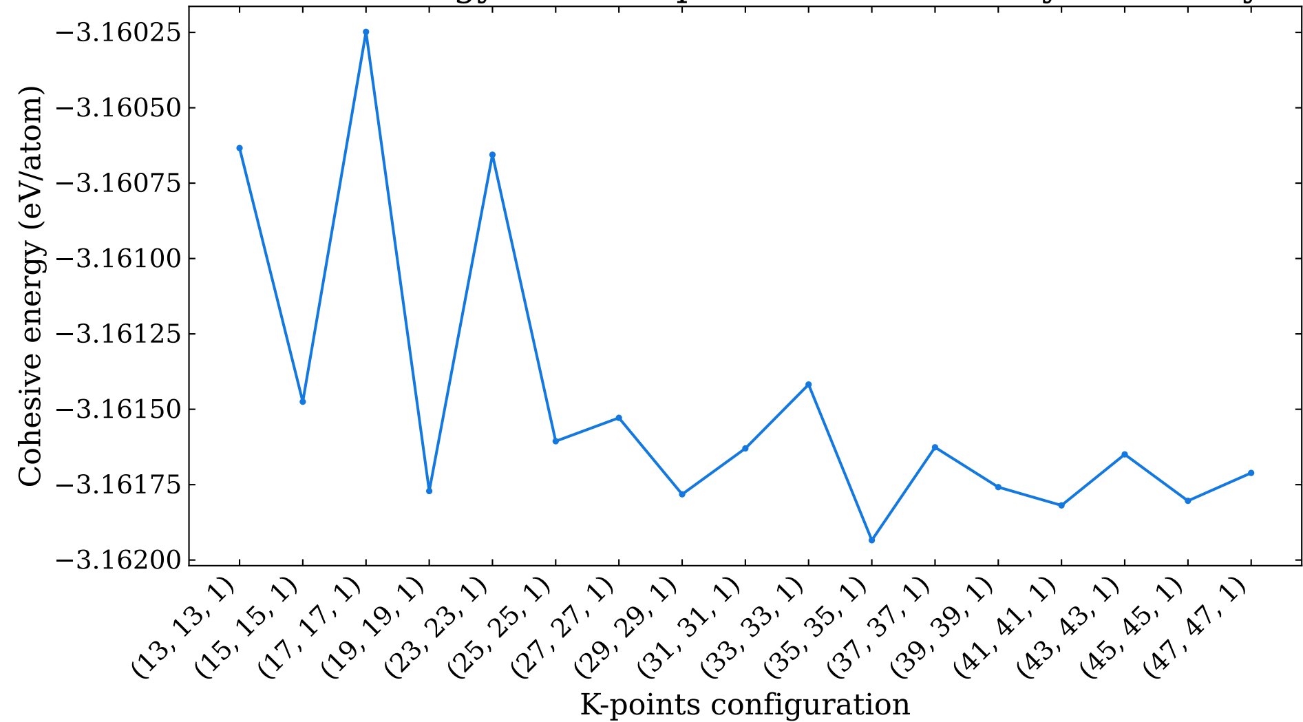
Cohesive energy versus k-points for cubic beryllene trilayer
