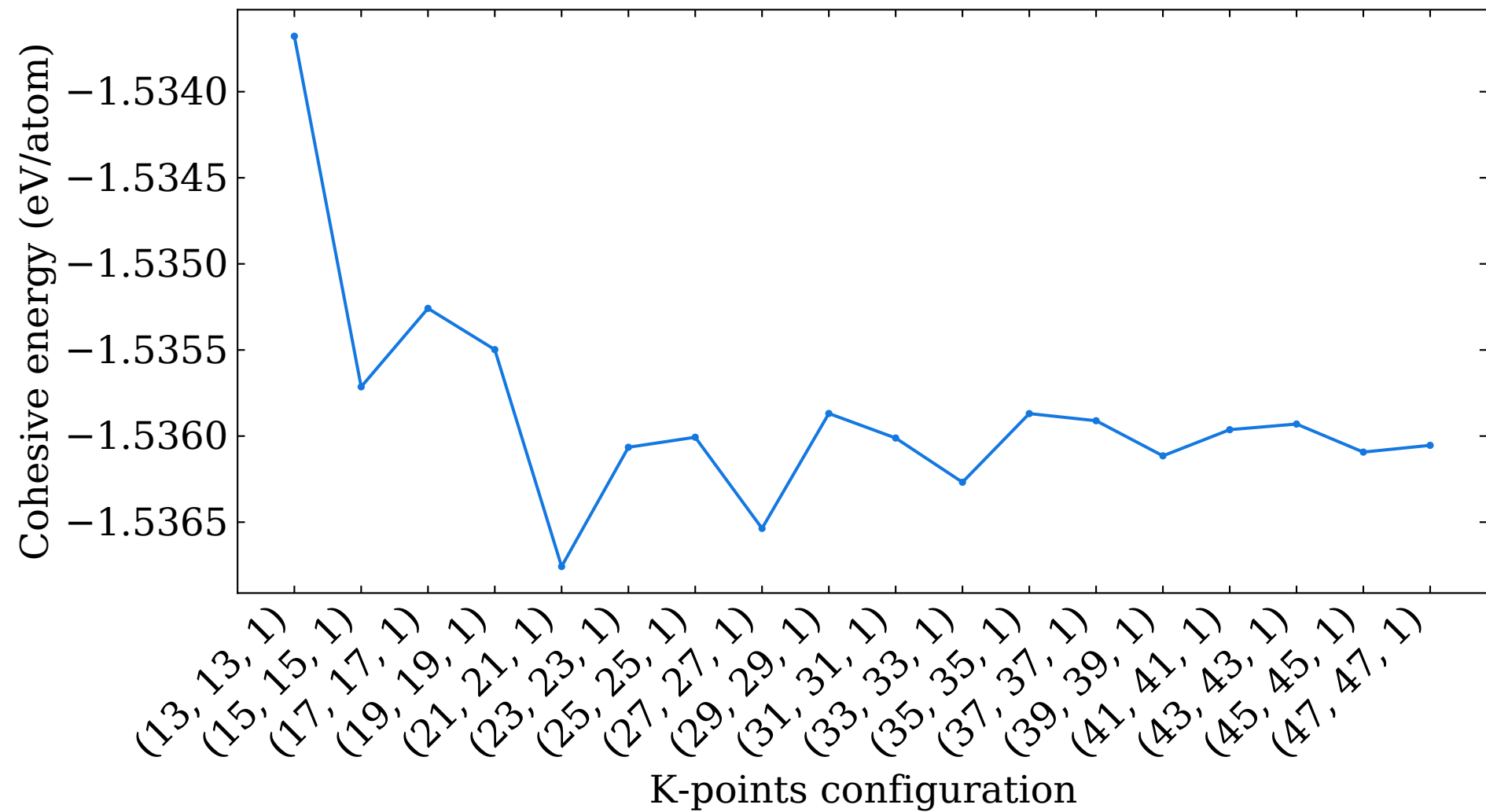
Cohesive energy versus k-points for graphic Beryllene monolayer
