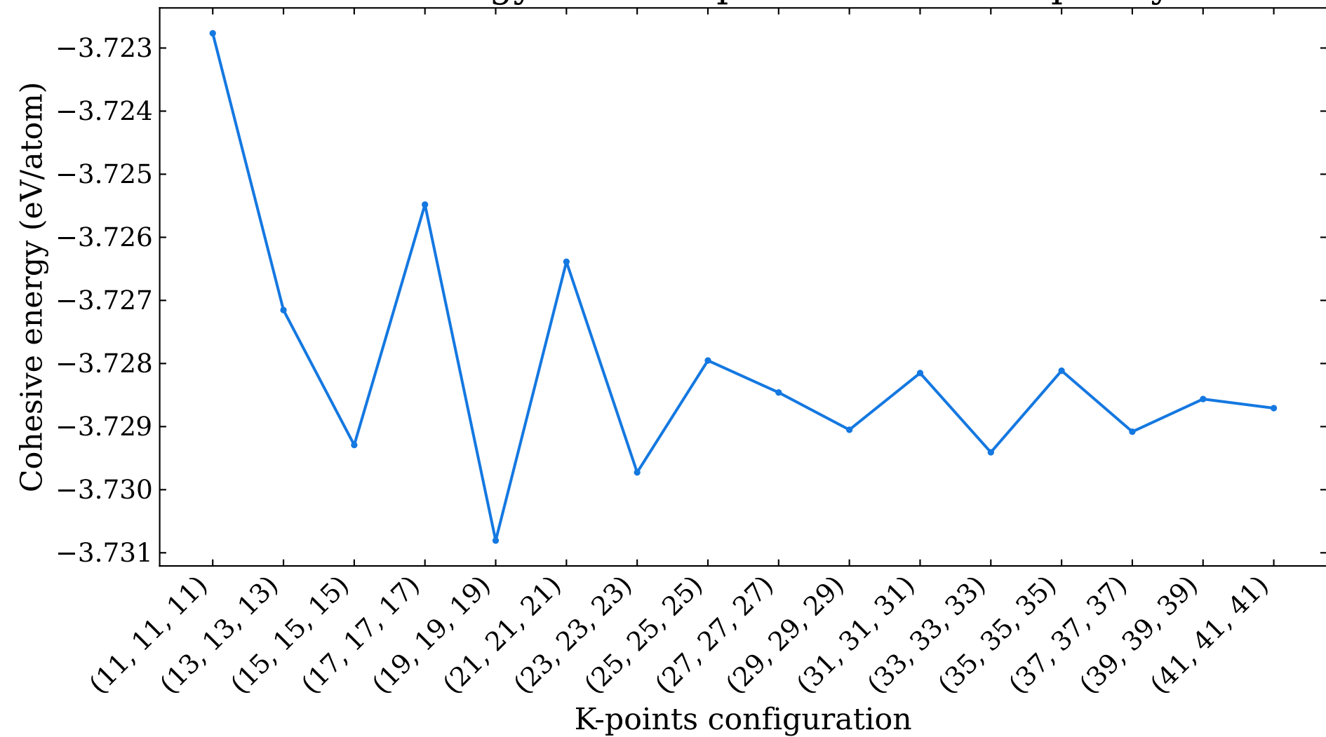
Cohesive energy versus k-points for bulk hcp beryllium
