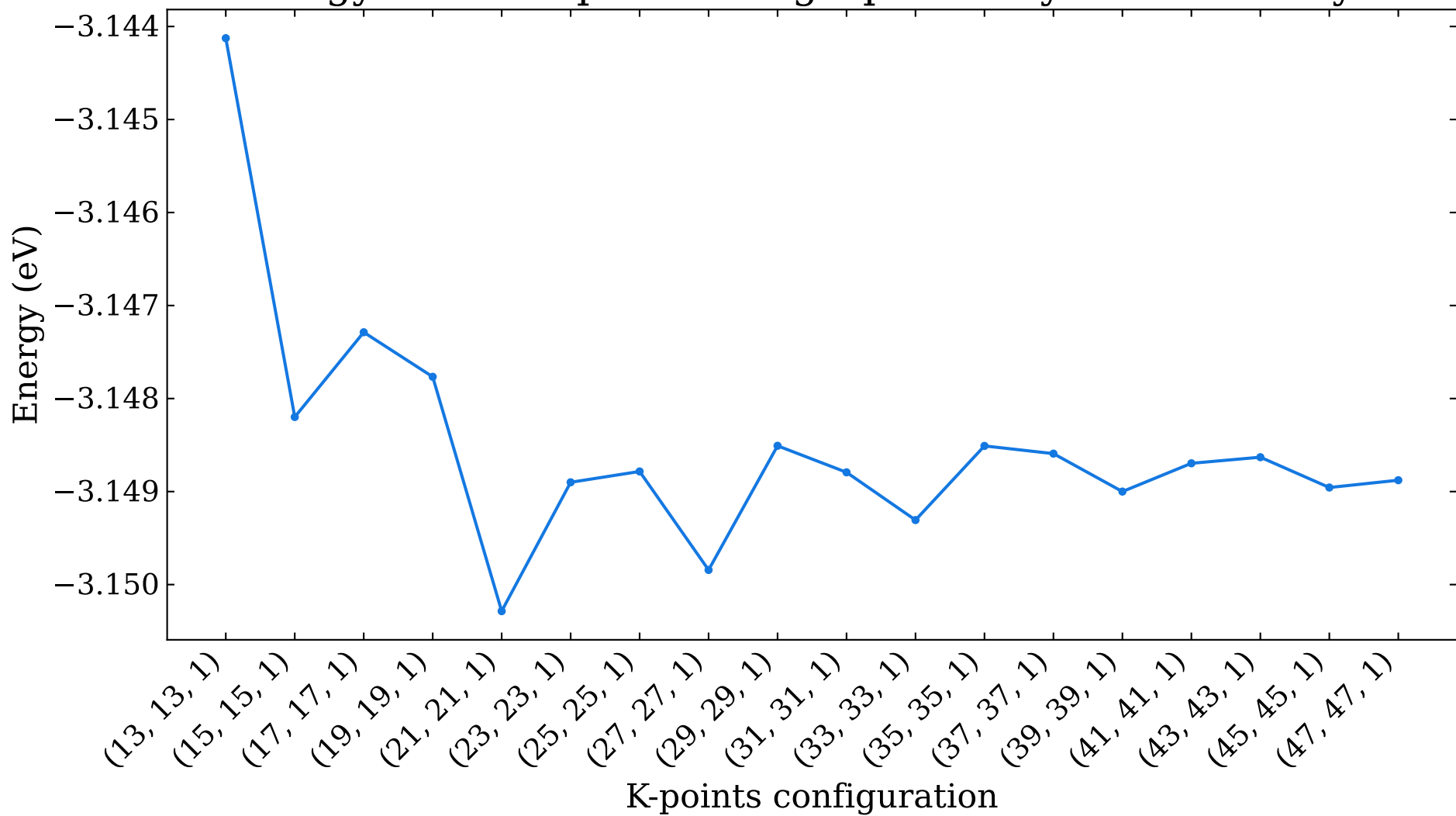
Energy versus k-points for graphic Beryllene monolayer
