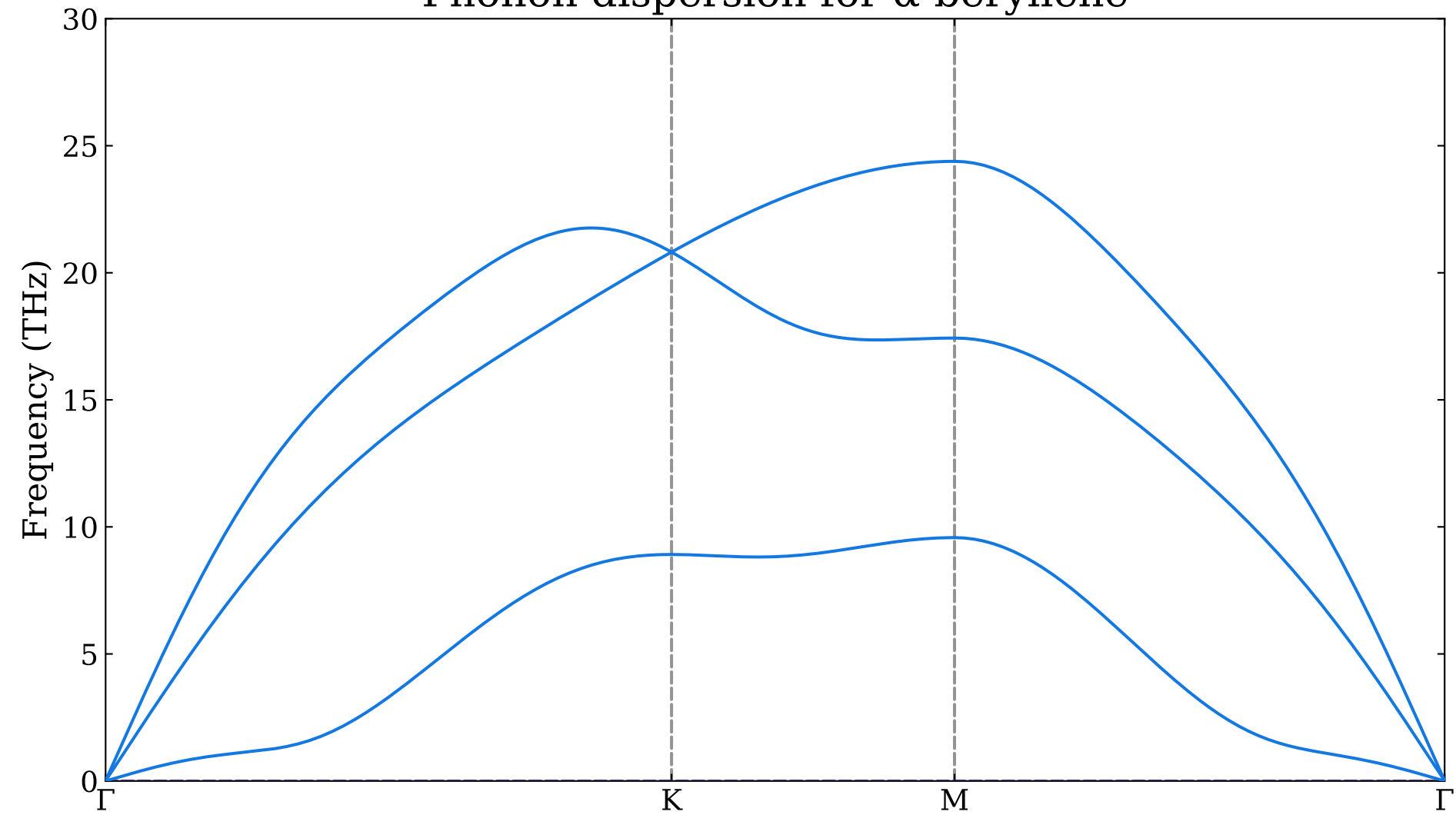
Phonon dispersion for \alpha -beryllene
