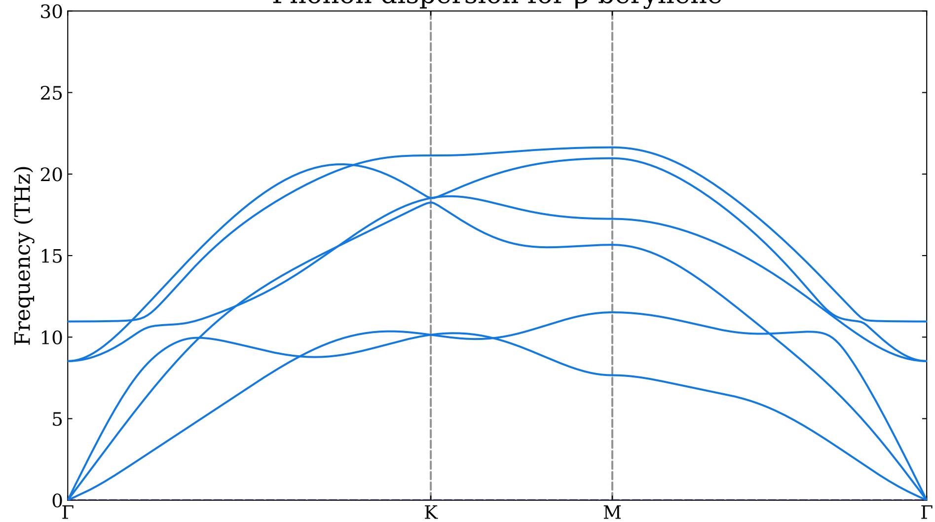
Phonon dispersion for \beta -beryllene
