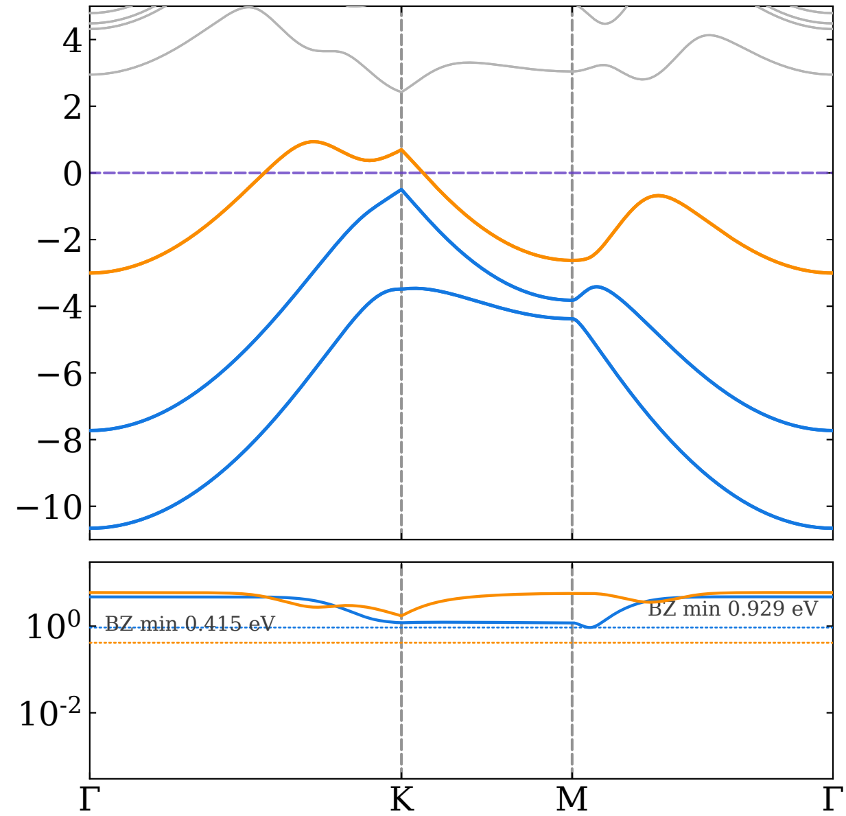
1H- \beta -beryllene: Z_2 = 0/0 (WCC)
