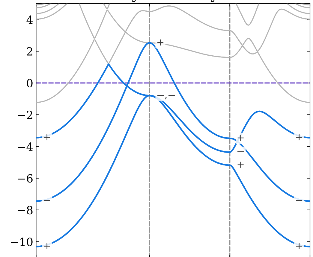
cubic beryllene trilayer: \nu = 1
