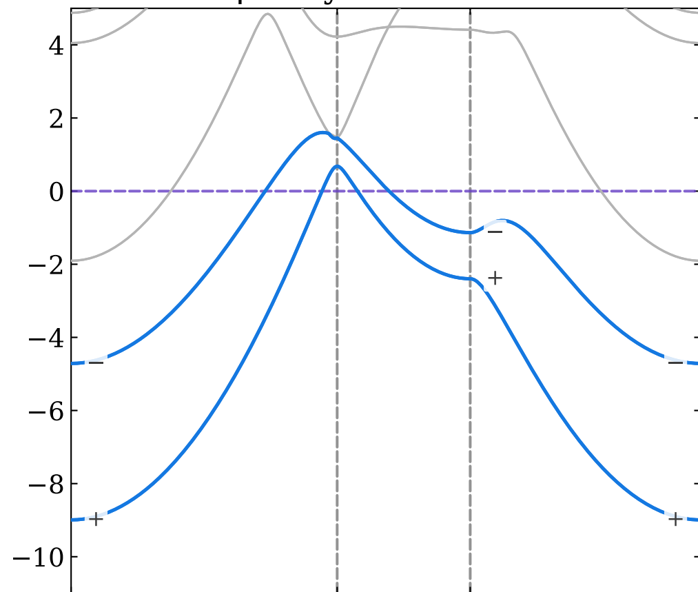
\beta -beryllene: \nu = 0
