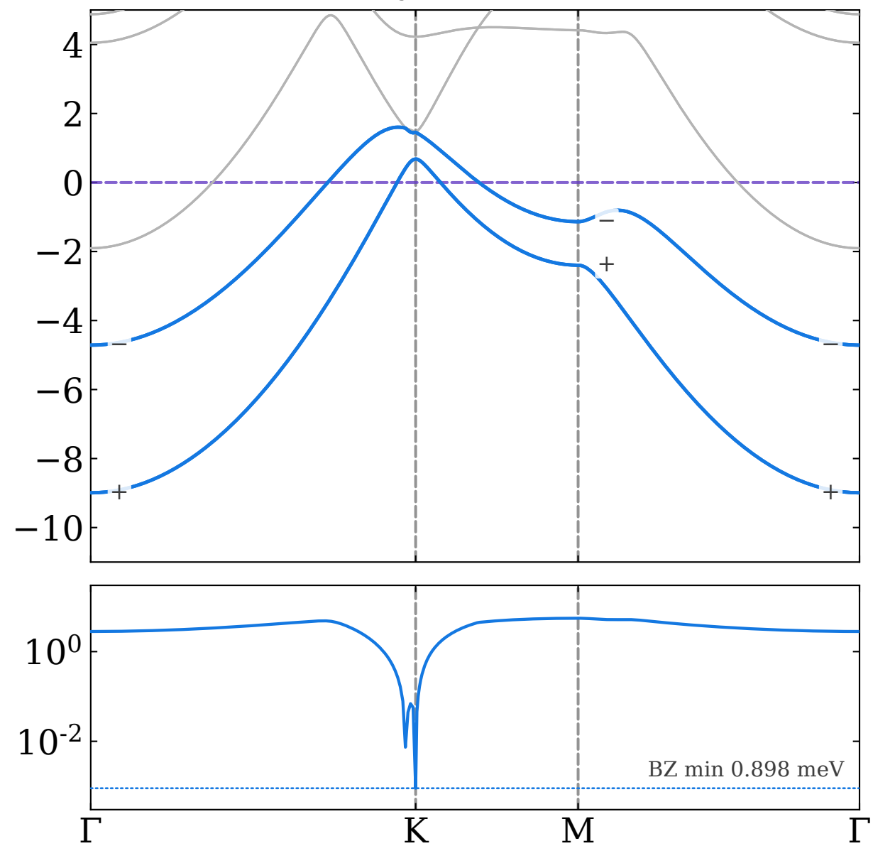
\beta -beryllene: \nu = 0
