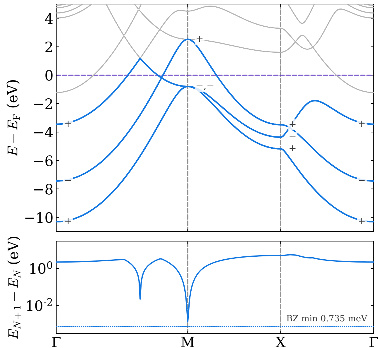
cubic beryllene trilayer: \nu = 1
