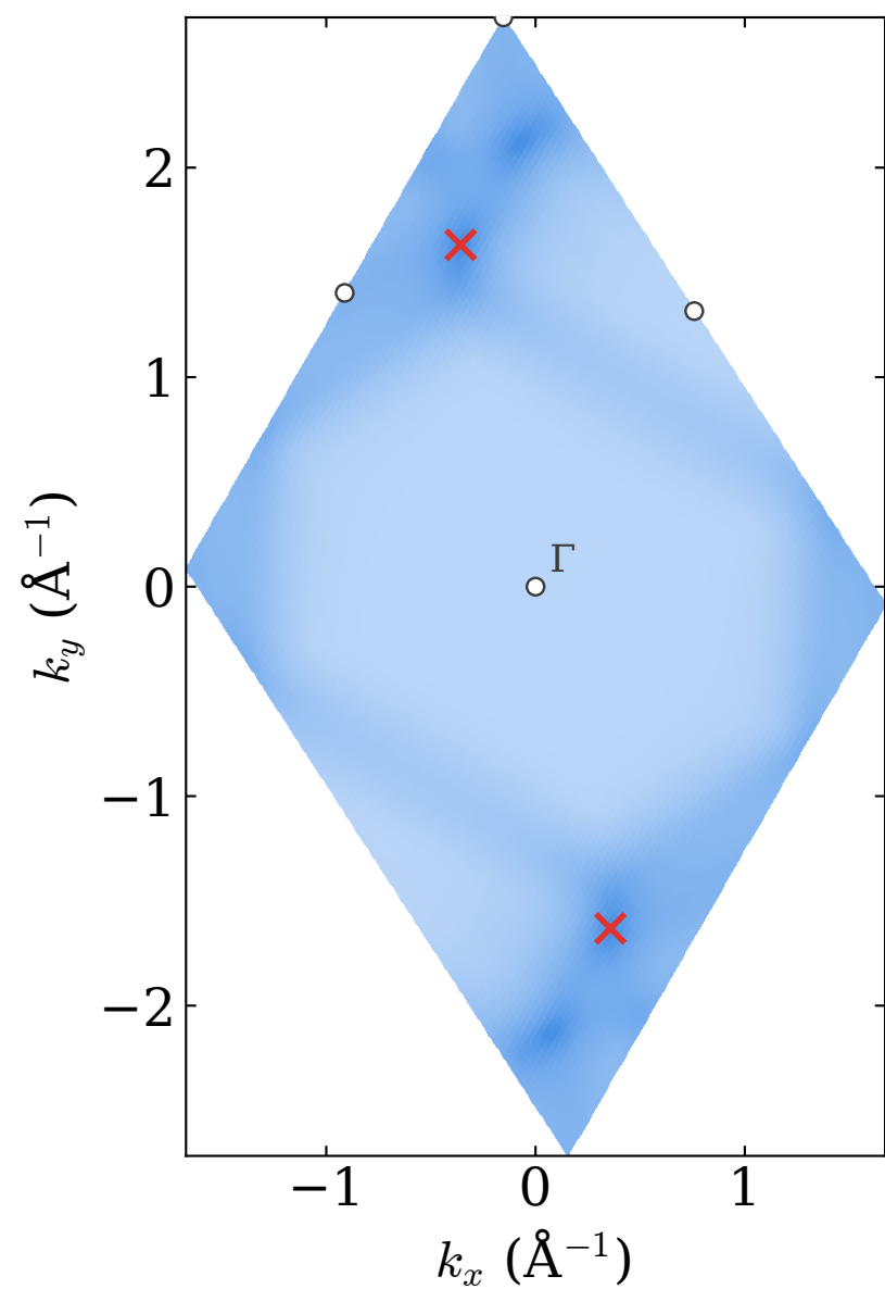
1H- \beta -beryllene, N = 6 min 0.415 eV
