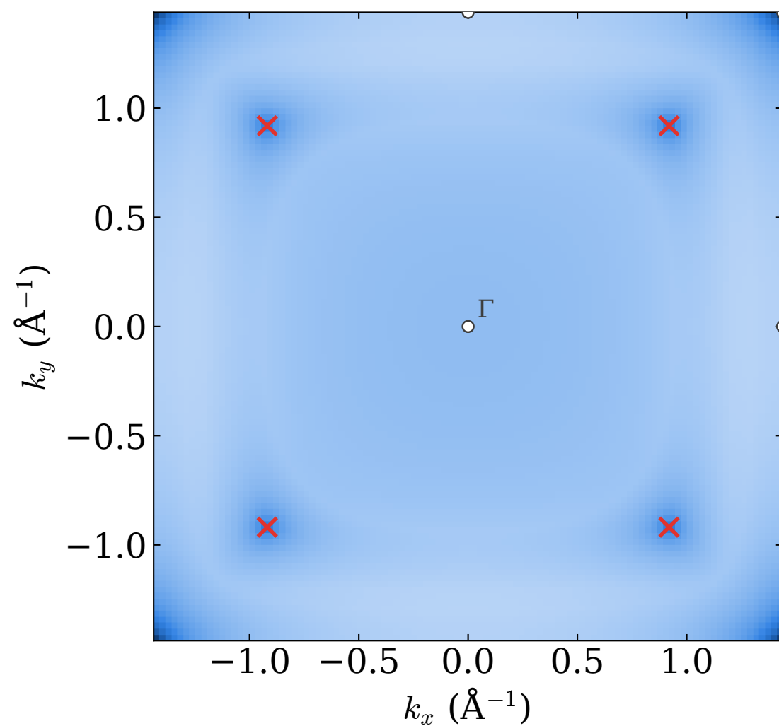
cubic beryllene trilayer, N = 6 min 0.735 meV
