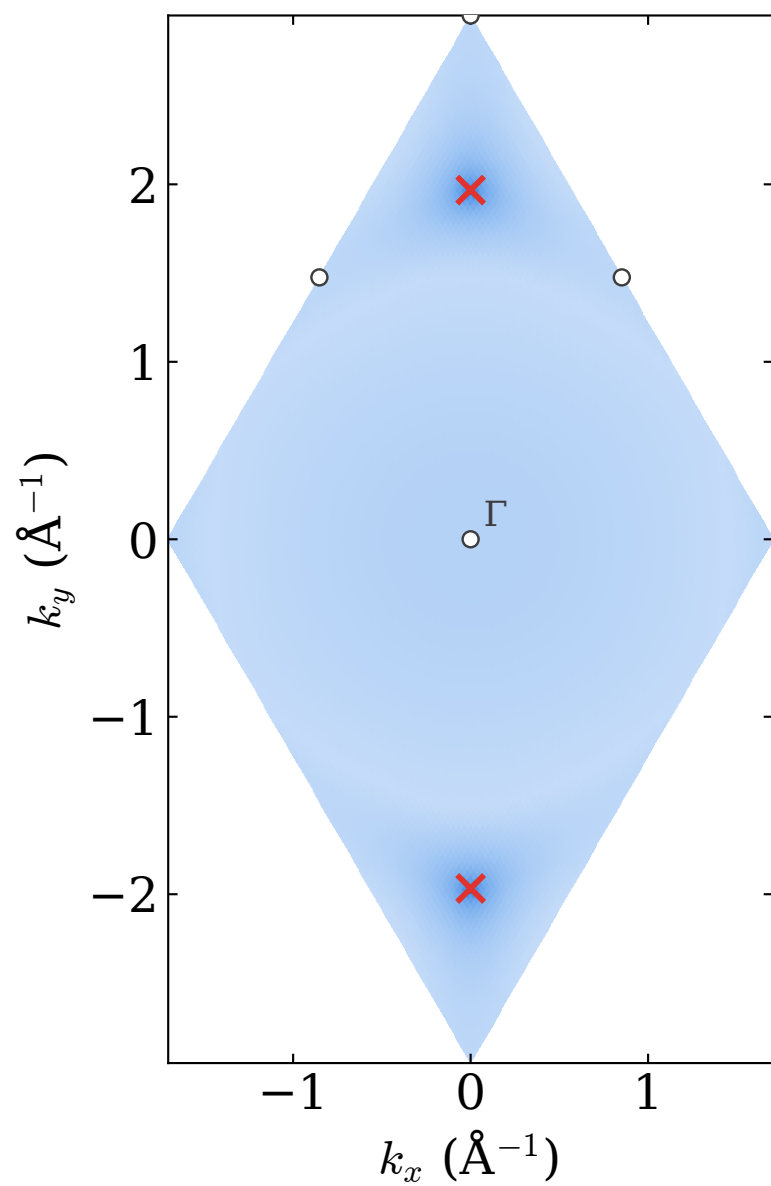
\alpha -beryllene, N = 2 min 1.13 meV
