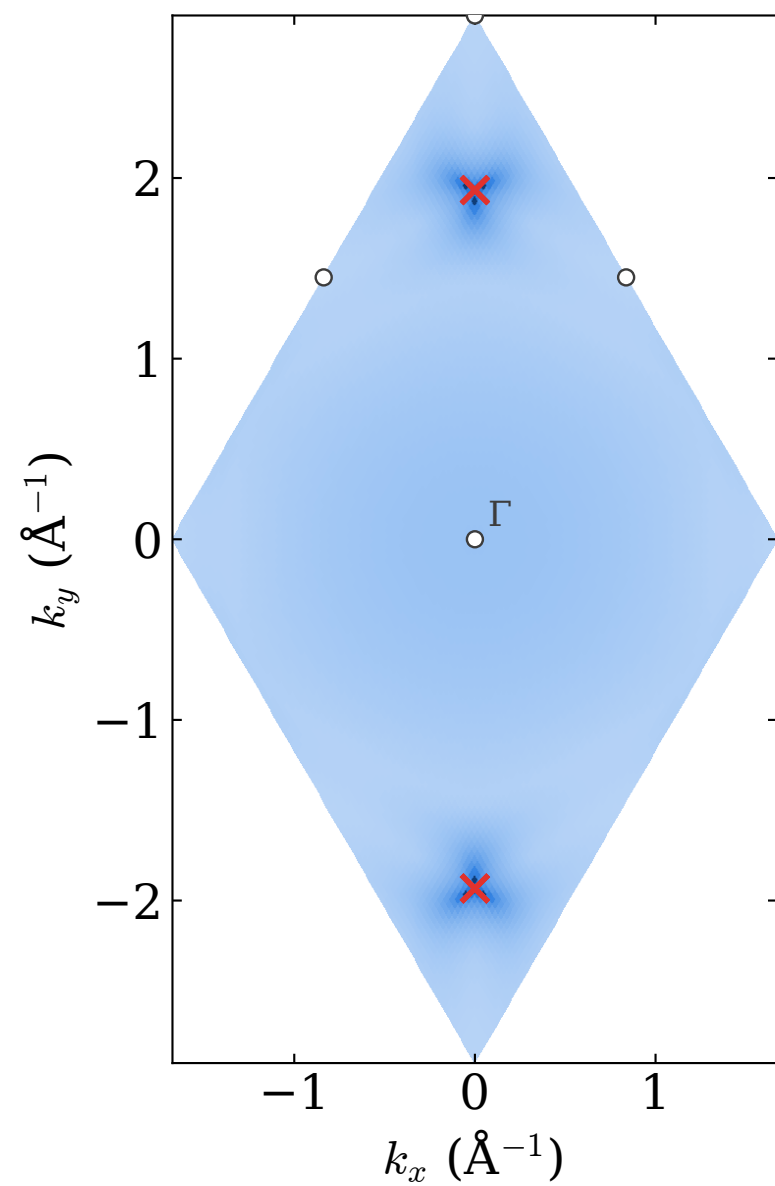
\beta -beryllene, N = 4 min 0.898 meV
