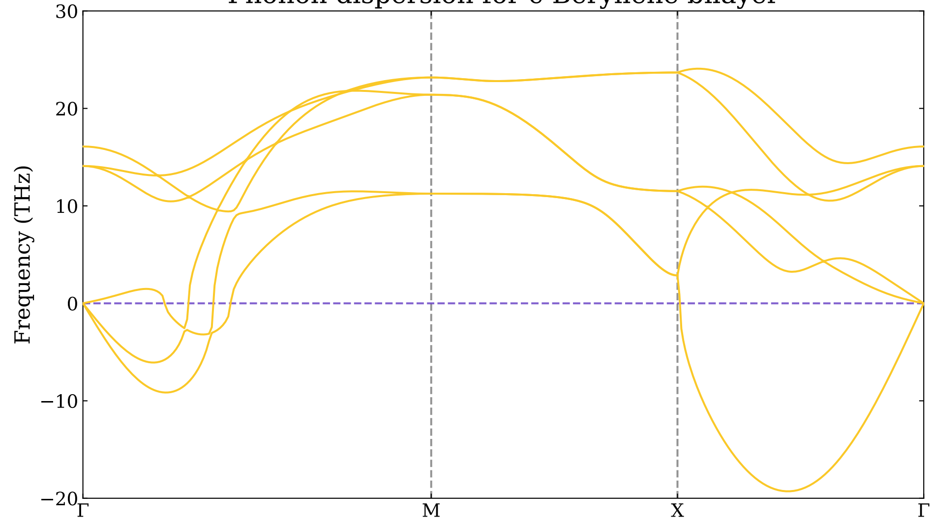
Phonon dispersion for c-Beryllene bilayer
