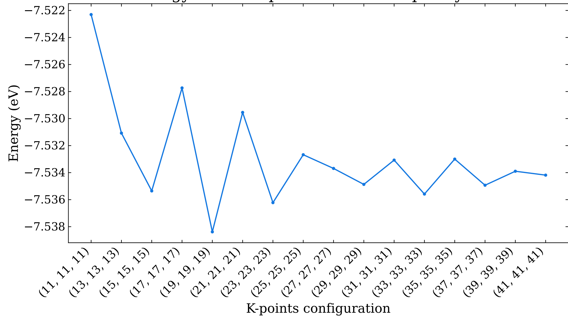
Energy versus k-points for bulk hcp beryllium
