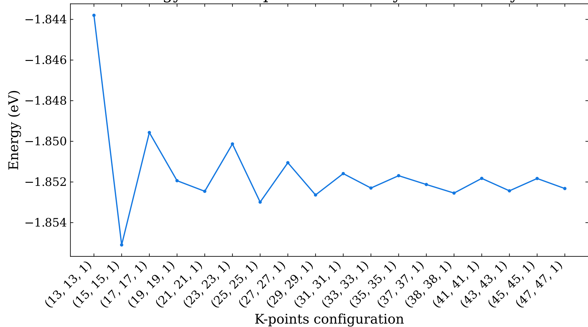
Energy versus k-points for c-beryllene monolayer
