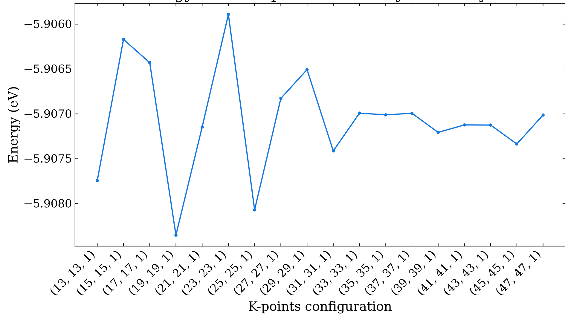
Energy versus k-points for c-beryllene bilayer
