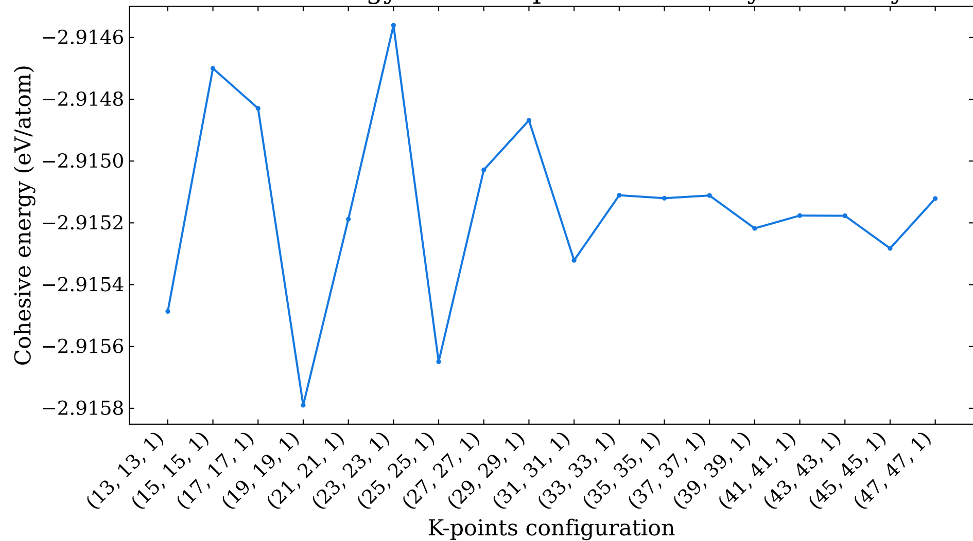
Cohesive energy versus k-points for c-beryllene bilayer
