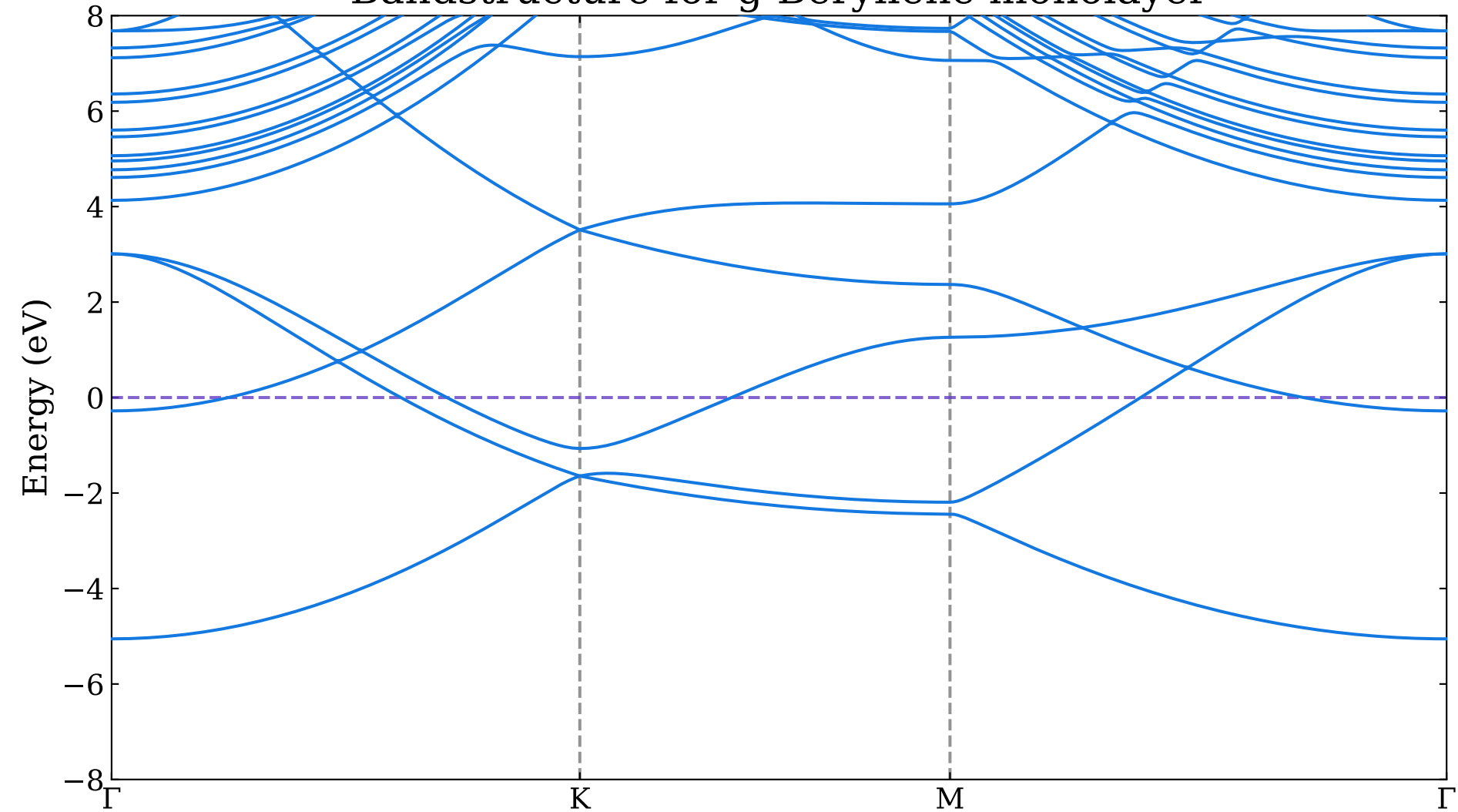
Bandstructure for g-Beryllene monolayer
