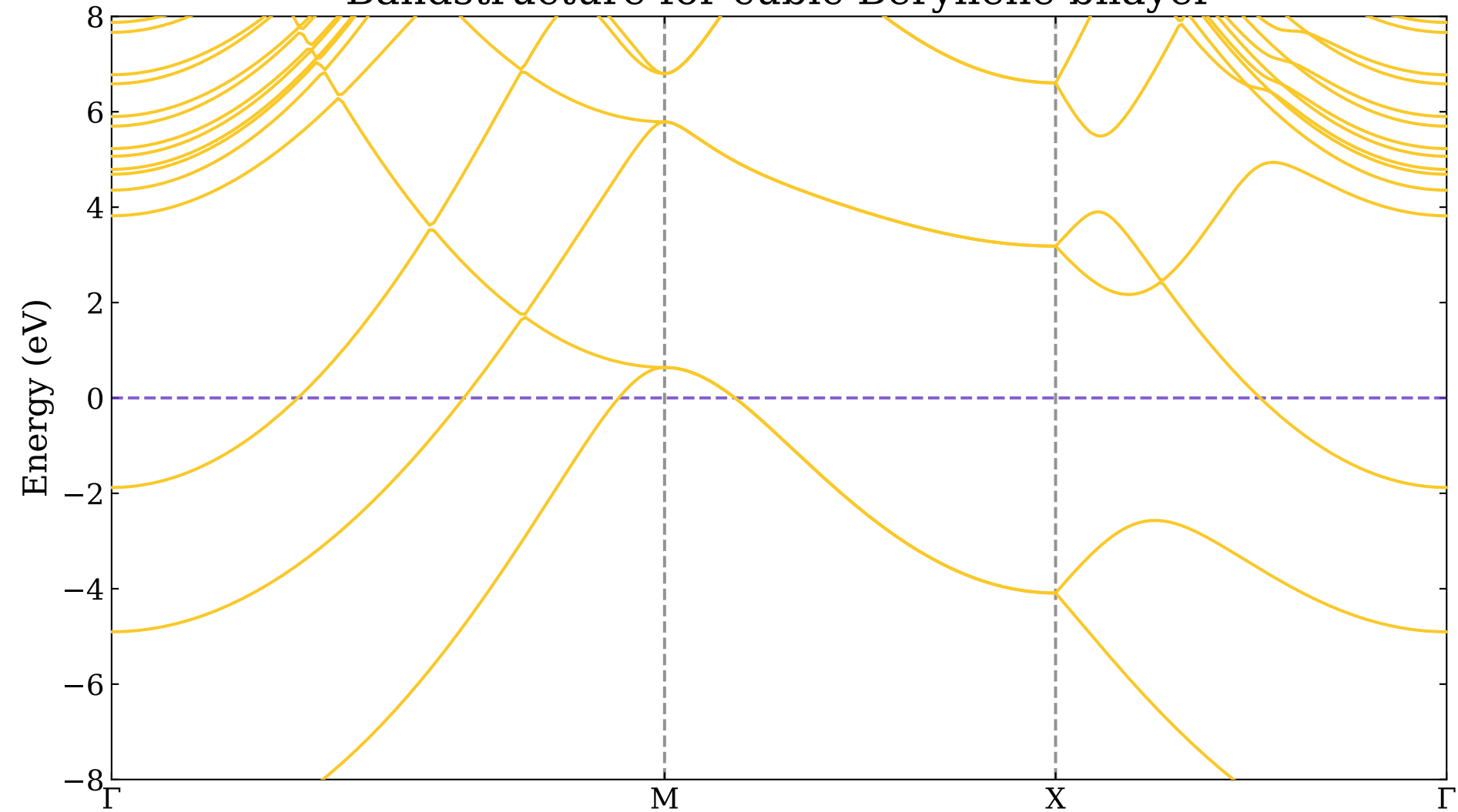
Bandstructure for cubic Beryllene bilayer
