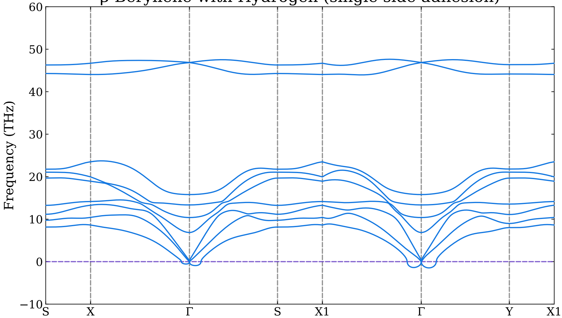
\beta -Beryllene with Hydrogen (single side adhesion)
