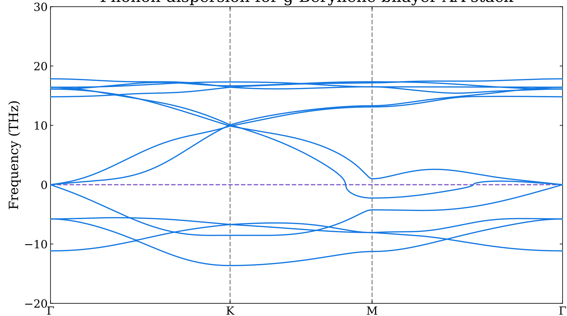
Phonon dispersion for g-Beryllene bilayer AA stack
