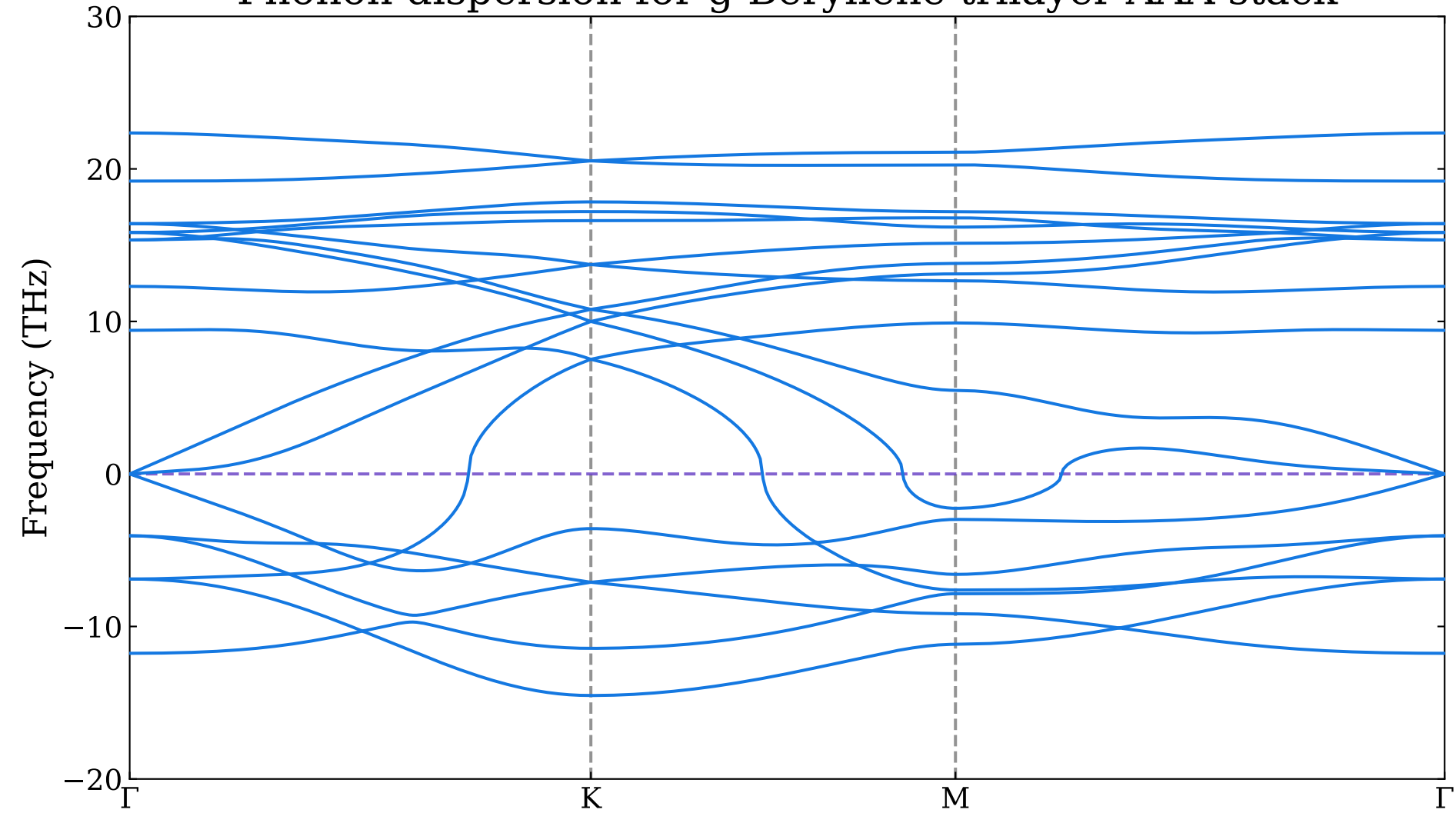
Phonon dispersion for g-Beryllene trilayer AAA stack
