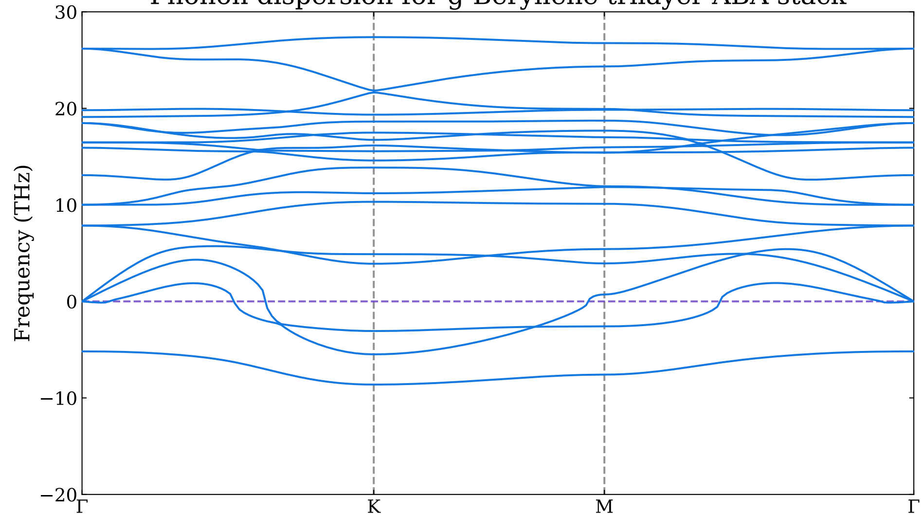
Phonon dispersion for g-Beryllene trilayer ABA stack
