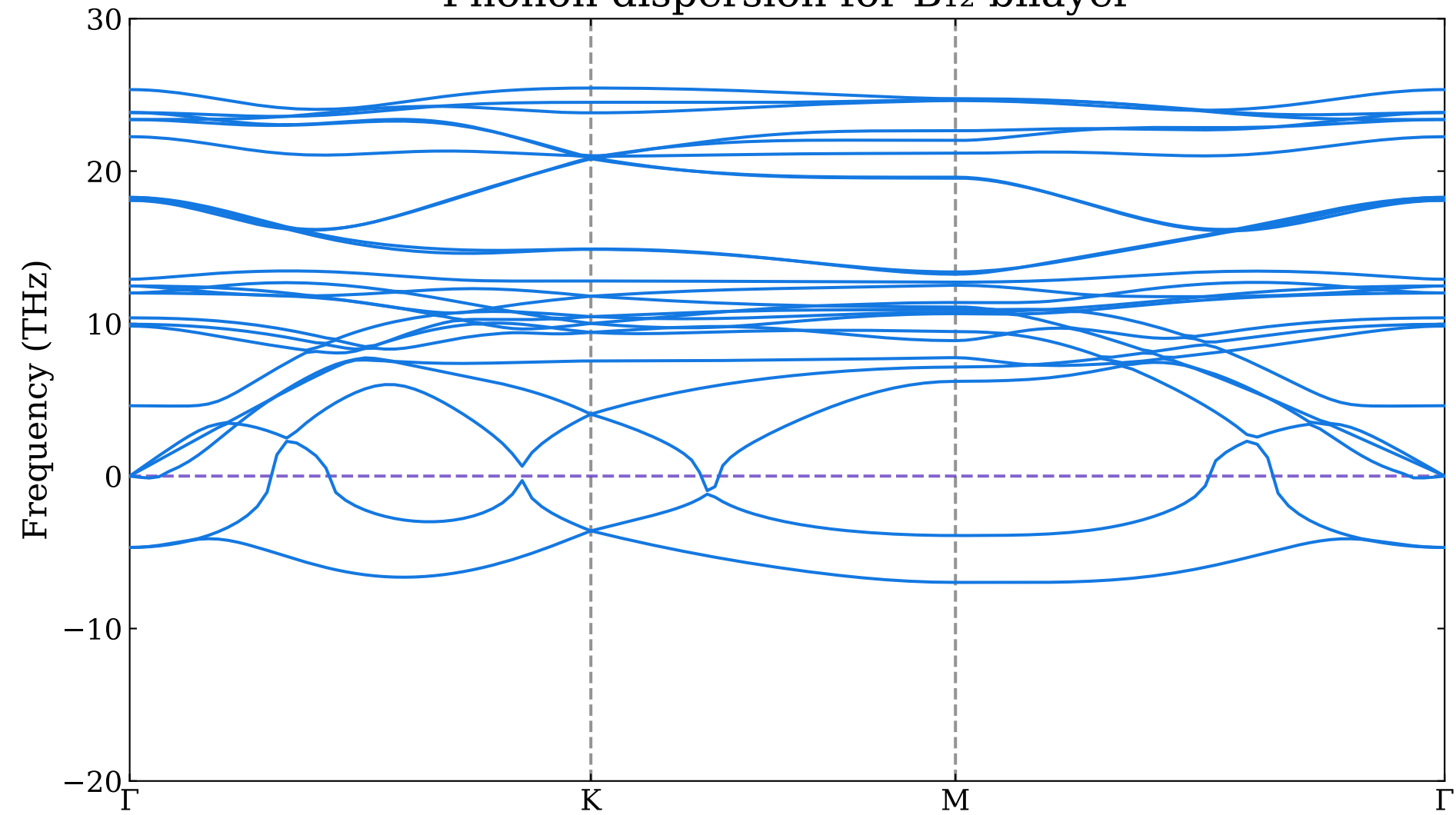
Phonon dispersion for B 12 bilayer
