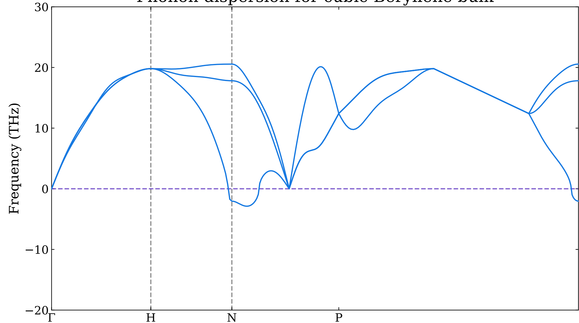
Phonon dispersion for cubic-Beryllene bulk
