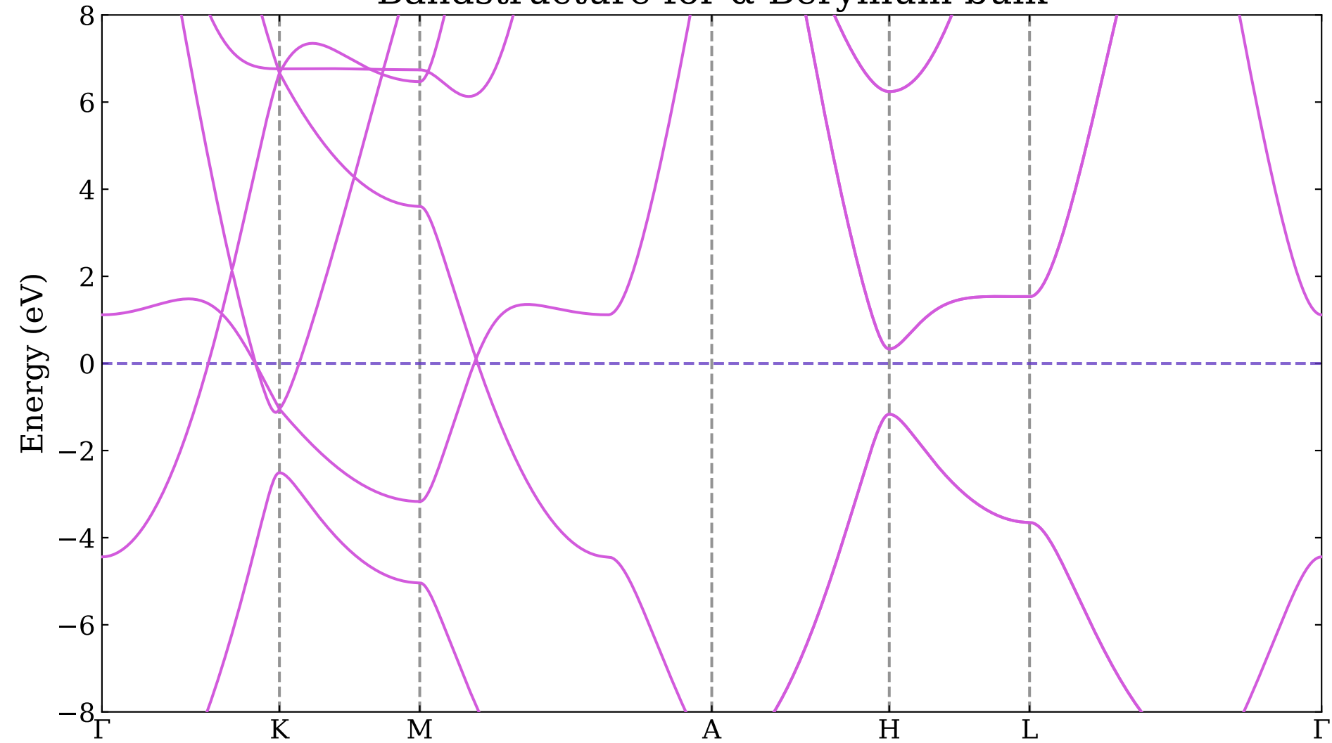
Bandstructure for \alpha -Beryllium bulk
